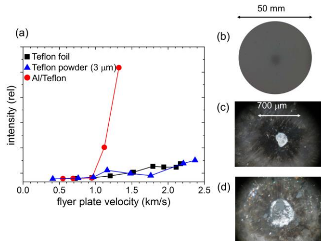
Fig. 6. (a) Total emission intensity from Al/Teflon and two forms of Teflon alone. Above 1 km/s, Al/Teflon initiation results in huge emission bursts. (b) Al/Teflon sample on a 2'' window. (c) Teflon powder after impact with 700 \mu\text{m} diameter flyer, shows dark debris spread out from the center which was vaporized. (d) Al/Teflon after impact has a debris field extending outward from the center, and much of the central region has been vaporized.
