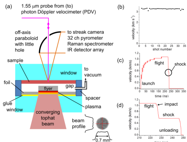
Fig. 1. Schematic of experiment for ns, \mu\text{m} resolution. A flattop laser beam (note beam profile) 0.7 mm in diameter, produced with a diffractive optic, launches a metal foil that flies across a gap to impact a sample. The flyer velocity is recorded by an optical interferometer (PDV). A parabolic mirror collects emission from the sample or brings in IR laser beams. (b) Reproducibility measurement where 33 flyers were shot from one assembly. (c) Velocity record where a 50 \mu\text{m} thick flyer was shot at 1.1 km/s onto a glass window. (d) Impact record on expanded scale. The velocity 0.55 km/s, lasting \sim 15 ns, is the speed U_p of the glass/foil interface.
