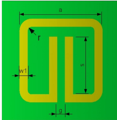
Figure 3.10: Square SSRR unit cell geometry on a 3mm x 3mm PCB substrate with the following static dimensions: a=2.5mm , g=w1=.2mm
