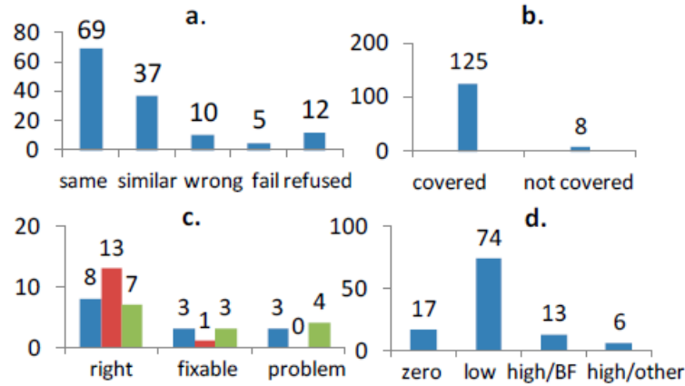
Figure 7: Validation results for the abstract syntax describing modeler navigation among evaluation abstraction patches. (a) How well the Wizard-of-Oz experimenter did at meeting participant requests in the “live” task during the experiment (b) How many of the abstractions in the study our abstract syntax covered (c) How well abstract syntax covered modelers needs in retrospect, judged by a panel of experts. (d) How expensive the navigations in the study would have been in a hypothetical interface designed around the abstract syntax.
