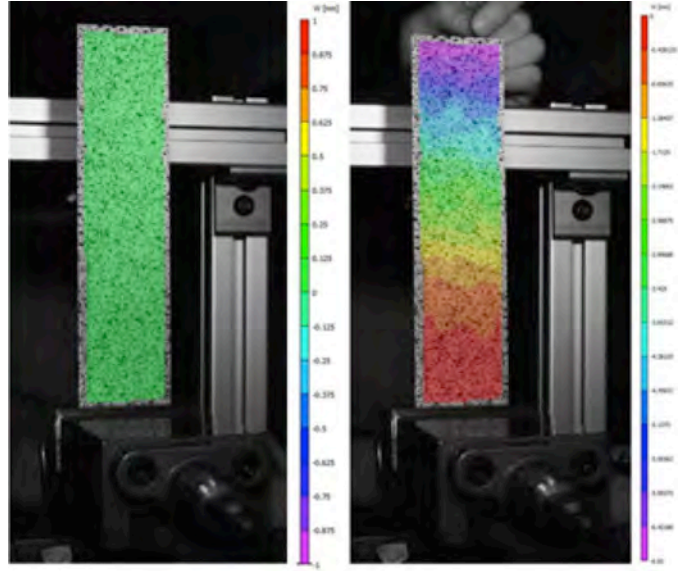
Figure 11 Left: initial image with zero displacement; right: the plate after it is released from an initial displacement of the corner
