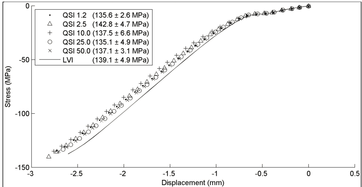
Figure 7. Comparison of stress vs. displacement for CAI of S2/SC-15 eight-ply, 102- x 152-mm, quasi-isotropic test samples. Each curve shows an average of five tests. LVI-tested samples were slightly stiffer under compression, while both QSI and LVI samples failed at a similar stress level.
