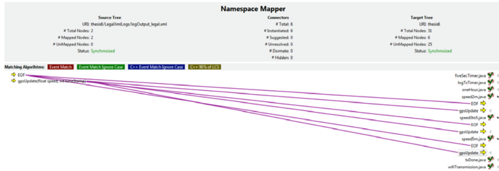
Figure 29. gpsUpdate-only mapping
