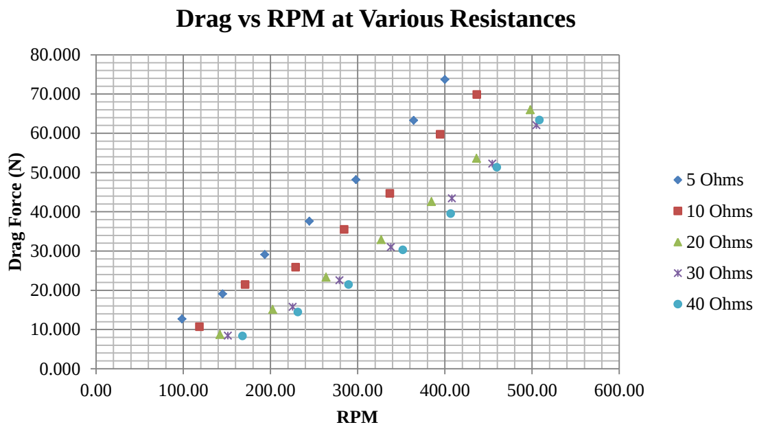
Figure 21. Drag force and RPM correlation at various resistances in the circuit for full turbine configuration.
