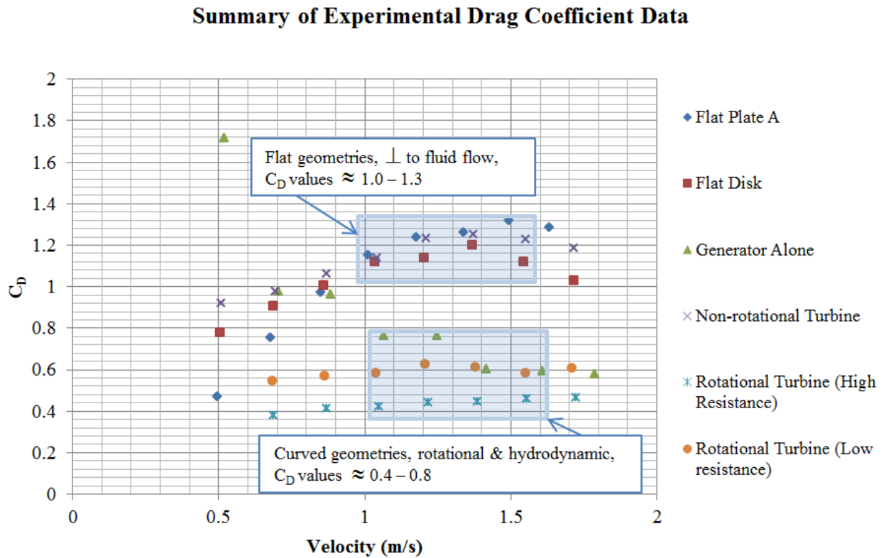
Figure 64. Summary of experimental drag coefficient calculations.
