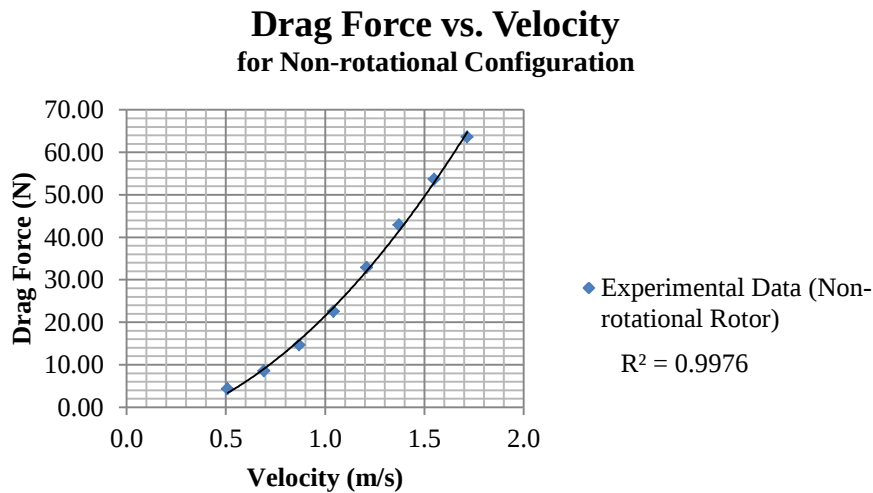
Figure 36. Trendline data for non-rotational full turbine configuration, drag force vs. velocity.
