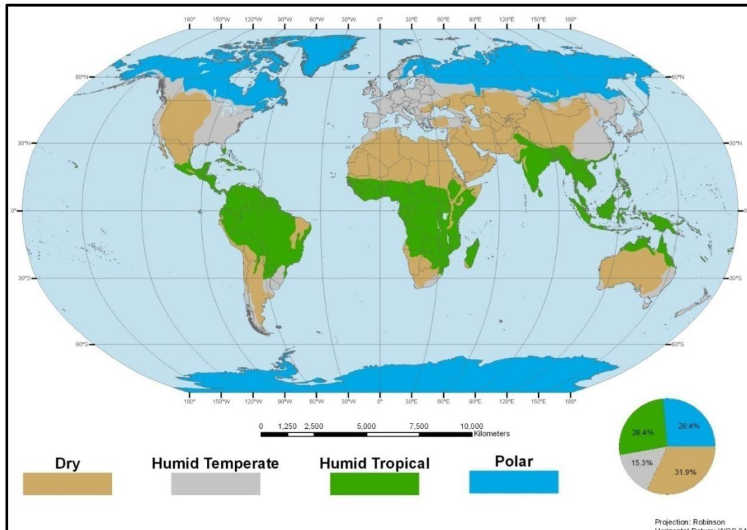
Figure 1. World climatic regions.
