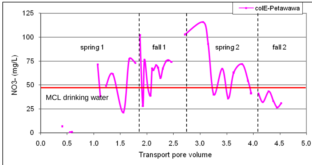
Figure 6-18. Nitrate ( \text{NO}_3^- ) effluent concentration as a function of transport pore volumes from Column E (Petawawa).
