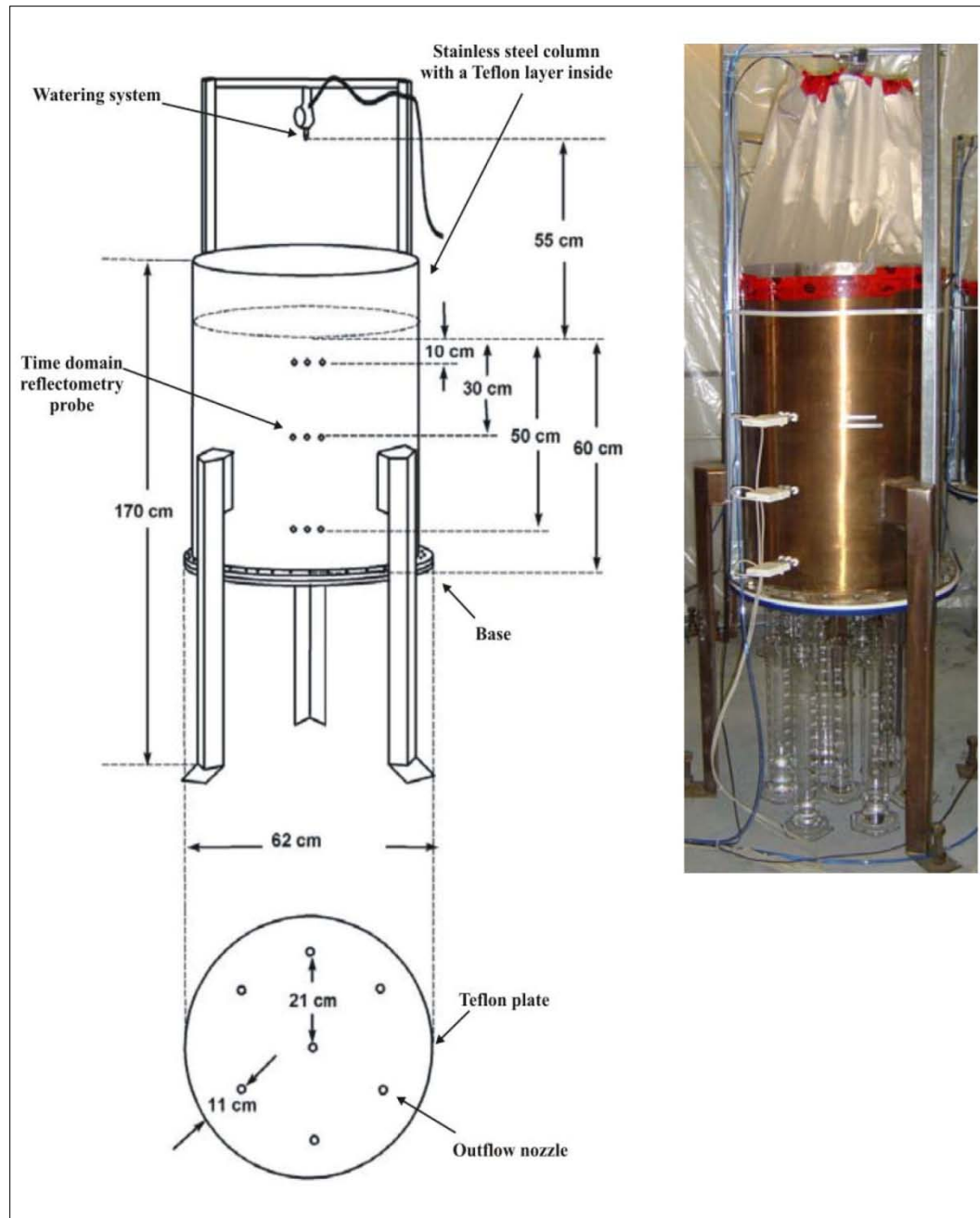
Figure 6-4. Dimensions of the sand columns.
