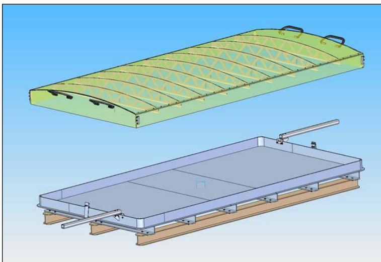
Figure 8-17. Schematic of the stainless steel burning table.
