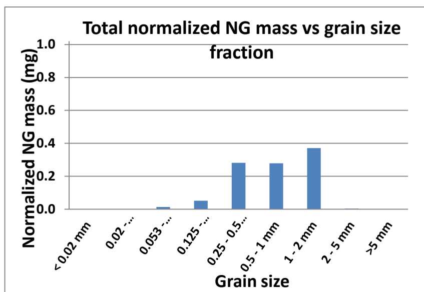
Figure 5-23. Total normalized NG mass in soil fractions (DRDC).
