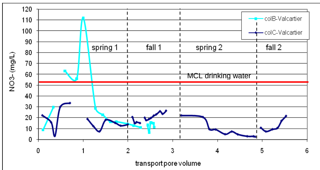
Figure 6-17. Nitrate ( \text{NO}_3^- ) effluent concentration as a function of transport pore volumes for Columns B and C of Valcartier.
