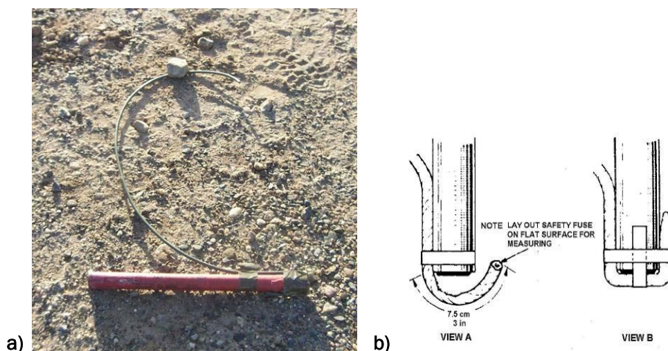
Figure 8-11. Typical flare with a safety fusee for ignition of the gun propellant: a) picture of the setup; b) schematic of preparing the railroad fusee for ignition.
