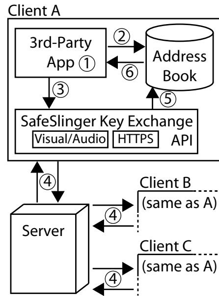
Figure 6: SafeSlinger secure key exchange API interaction.
