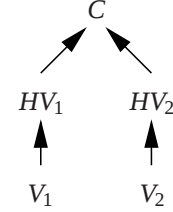
Figure 1: Multi-value commitment structure for authenticating and disclosing either V_1 or V_2 .
