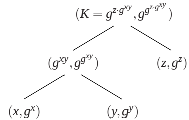
Figure 2: Group DH key agreement tree for 3 members (mod p operations omitted for clarity). The notation is (priv, pub), where the first element in the parenthesis lists the DH private key, and the second lists the DH public key. The group key is the private key K at the root.
