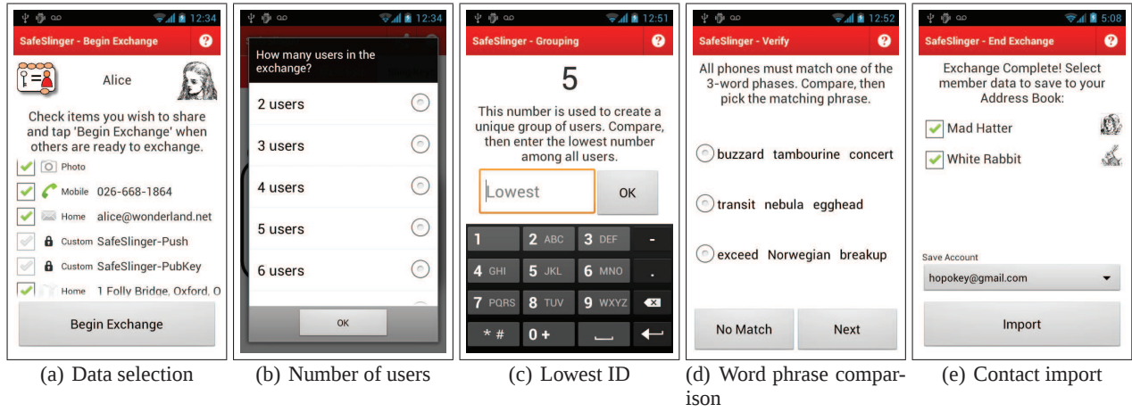
Figure 5: Secure contact information exchange sequence.
