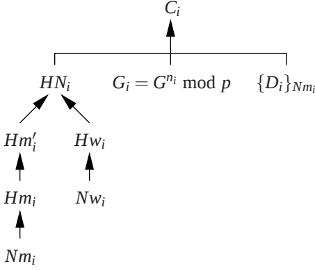
Figure 4: Multi-value commitment structure for user U_i . C_i , HN_i , Hm'_i , Hw_i , Hm_i , Nw_i , Nm_i , are 160-bit values; G_i is 512 bits, and D_i varies in length.
