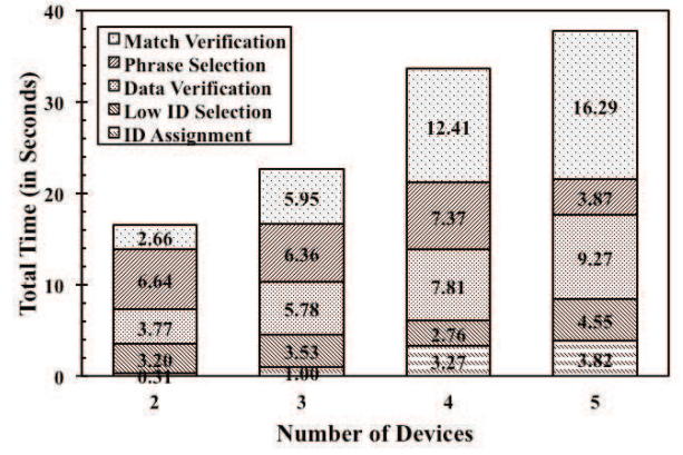
Figure 8: Time consumed during a SafeSlinger exchange.
