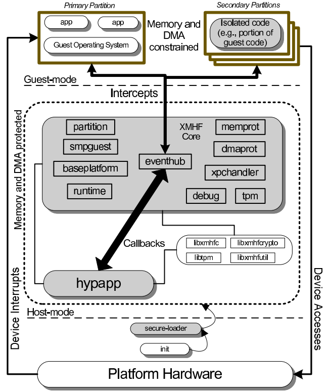
Figure 3: XMHF detailed architecture
