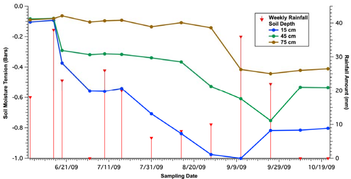
Figure 6-H Mean Soil Tensiometer Readings for Blocks 9-10 as a Function of Date and Soil Depth Together with Weekly Rainfall Amounts, Oxford Station. (Soil depths are referenced to the top of the soil mounds).
