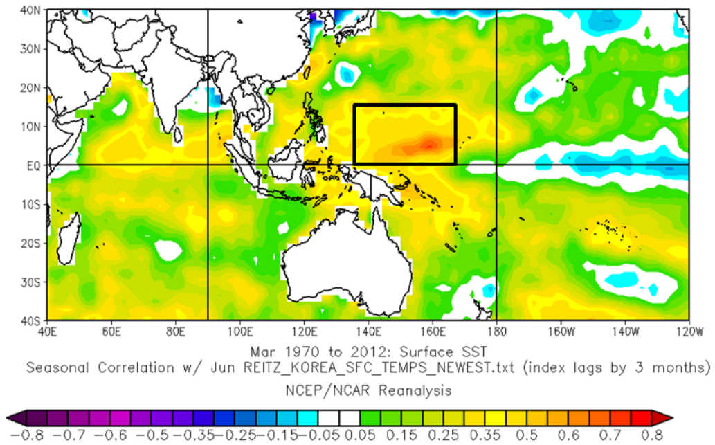
Figure 94. SST_TJUN3, used as a predictor for Jun surface air temperatures.
