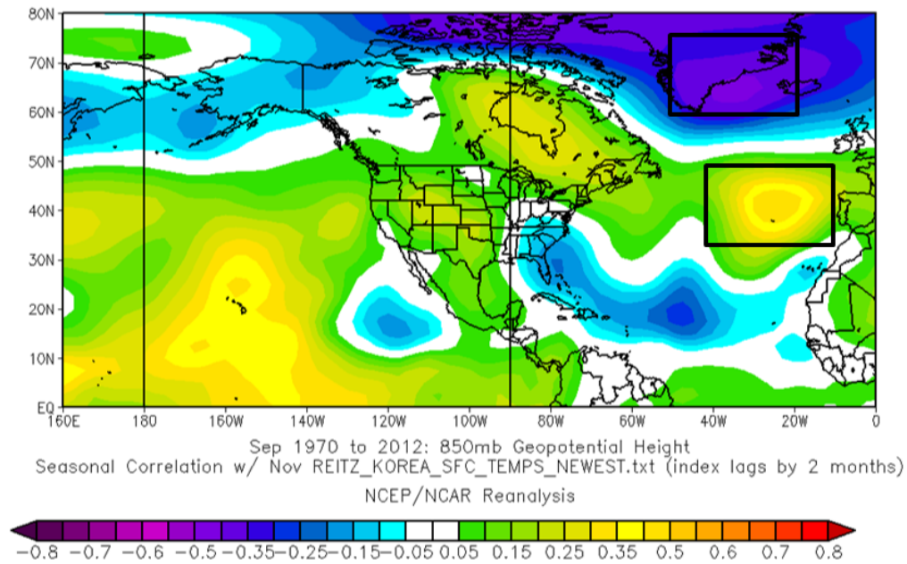
Figure 116. Inputs for KTI_NOV2, used as a predictor for Nov surface air temperatures.
