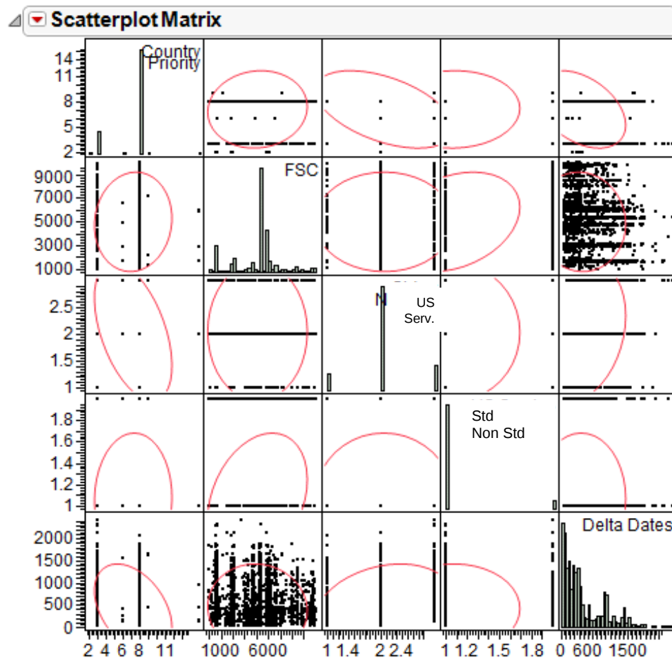
Figure 4.12 Multivariate pairwise estimation JMP® V9
