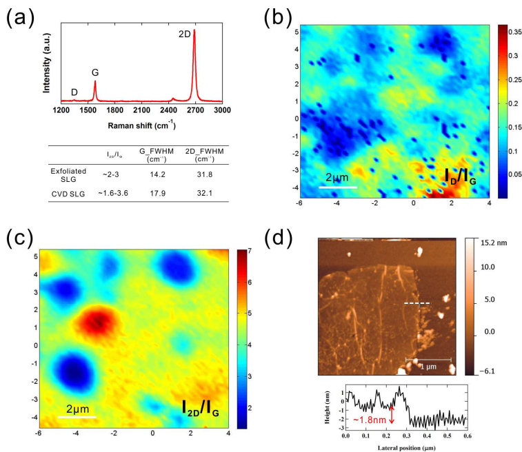
Fig. 2. Characterizations of transferred CVD graphene film on Si substrate with ~300 nm thermal oxide by Raman spectroscopy and AFM. (a) A representative Raman spectrum of CVD SLG measured in ambient using a 532 nm excitation laser. Inset: The I_{2D}/I_G , the G -band FWHM and 2D -band FWHM for exfoliated SLG 45 and CVD-grown SLG. (b) Raman mapping of I_D/I_G over a 10 × 10 μm 2 area. (c) Raman mapping of I_{2D}/I_G of a 10 × 10 μm 2 area, most (~> 80%) of which can be associated with SLG ( I_{2D}/I_G > 2 ). (d) AFM height image and profile of a transferred CVD graphene film. The height profile is recorded along the white dashed line indicated in the AFM image.
