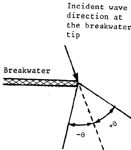
Figure 2. Definition sketch for using the random wave diffraction method of Goda (1985)
