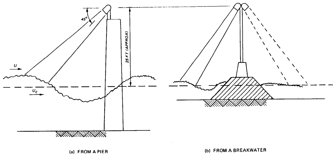
Figure 1. Schematic of Microwave Scatterometer used to Measure Surface Currents ( U_c ) and Wave Orbital Velocities ( U )
