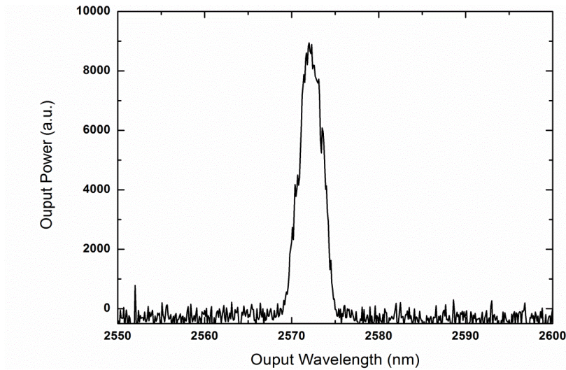
Figure 6. Laser output spectrum with peak at 2572.1 nm. FWHM of the peak is 3.1 nm
