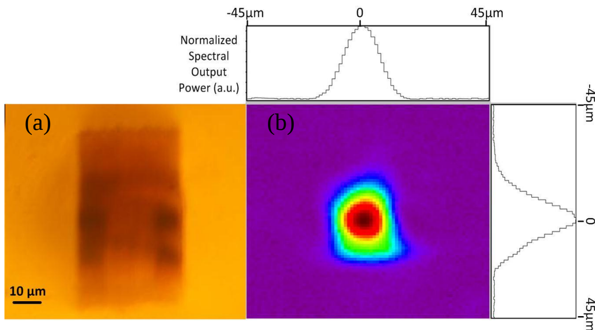
Figure 1. (a) Waveguide end facet cross-section (b) false color intensity profile of associated mode at 3.39 μm. Field of view is 90 x 90 μm.
