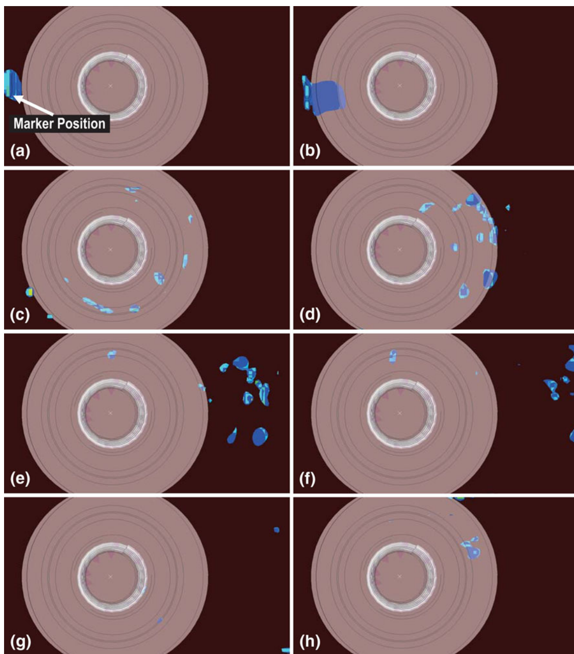
Fig. 9 Top view of the spatial distribution and temporal evolution of the marker-material (initially located on the workpiece interface/top-layer) volume fraction (red greater than 0.8, blue less than 0.2): tool rotation speed = 500 rpm; tool travel speed = 0.0025 m/s; tool tilt angle = 2.5°; tool plunge depth = 0.0001 m; 10 mm upper-diameter tool pin; welding time in seconds: (a) 2.7, (b) 6.6, (c) 10.5, (d) 14.4, (e) 18.3, (f) 22.2, (g) 26.1, (h) 30
