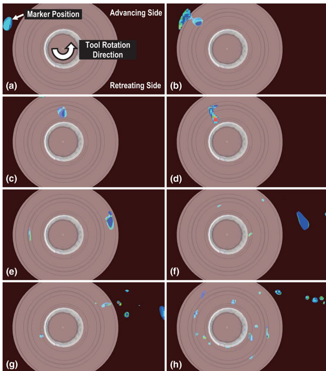
Fig. 6 Top view of the spatial distribution and temporal evolution of the marker-material (initially located on the workpiece advancing-side/top-layer) volume fraction (red greater than 0.8, blue less than 0.2); tool rotation speed = 500 rpm; tool travel speed = 0.0025 m/s; tool tilt angle = 2.5°; tool plunge depth = 0.0001 m; 10 mm upper-diameter tool pin; welding time in seconds: (a) 2.7, (b) 6.6, (c) 10.5, (d) 14.4, (e) 18.3, (f) 22.2, (g) 26.1, (h) 30
