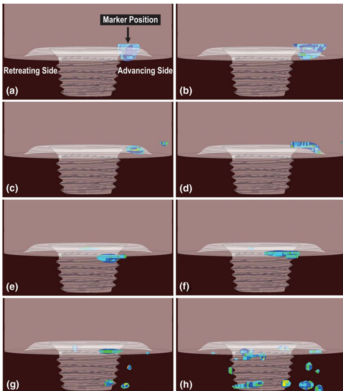
Fig. 7 Rear view of the spatial distribution and temporal evolution of the marker-material (initially located on the workpiece advancing-side/top-layer) volume fraction (red greater than 0.8, blue less than 0.2): tool rotation speed = 500 rpm; tool travel speed = 0.0025 m/s; tool tilt angle = 2.5°; tool plunge depth = 0.0001 m; 10 mm upper-diameter tool pin; welding time in seconds: (a) 2.7, (b) 6.6, (c) 10.5, (d) 14.4, (e) 18.3, (f) 22.2, (g) 26.1, (h) 30
