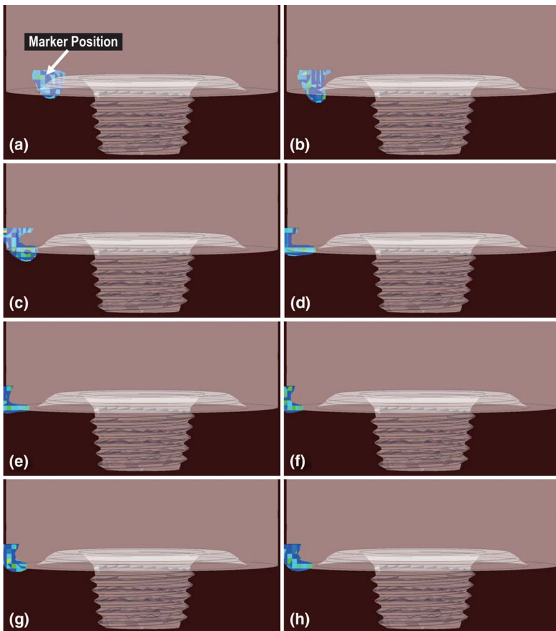
Fig. 13 Rear view of the spatial distribution and temporal evolution of the marker-material (initially located on the workpiece retreating side/top-layer) volume fraction (red greater than 0.8, blue less than 0.2): tool rotation speed = 500 rpm; tool travel speed = 0.0025 m/s; tool tilt angle = 2.5°; tool plunge depth = 0.0001 m; 10 mm upper-diameter tool pin; welding time in seconds: (a) 3.9, (b) 5.4, (c) 7.2, (d) 8.4, (e) 9.9, (f) 11.4, (g) 12.9, (h) 14.4
