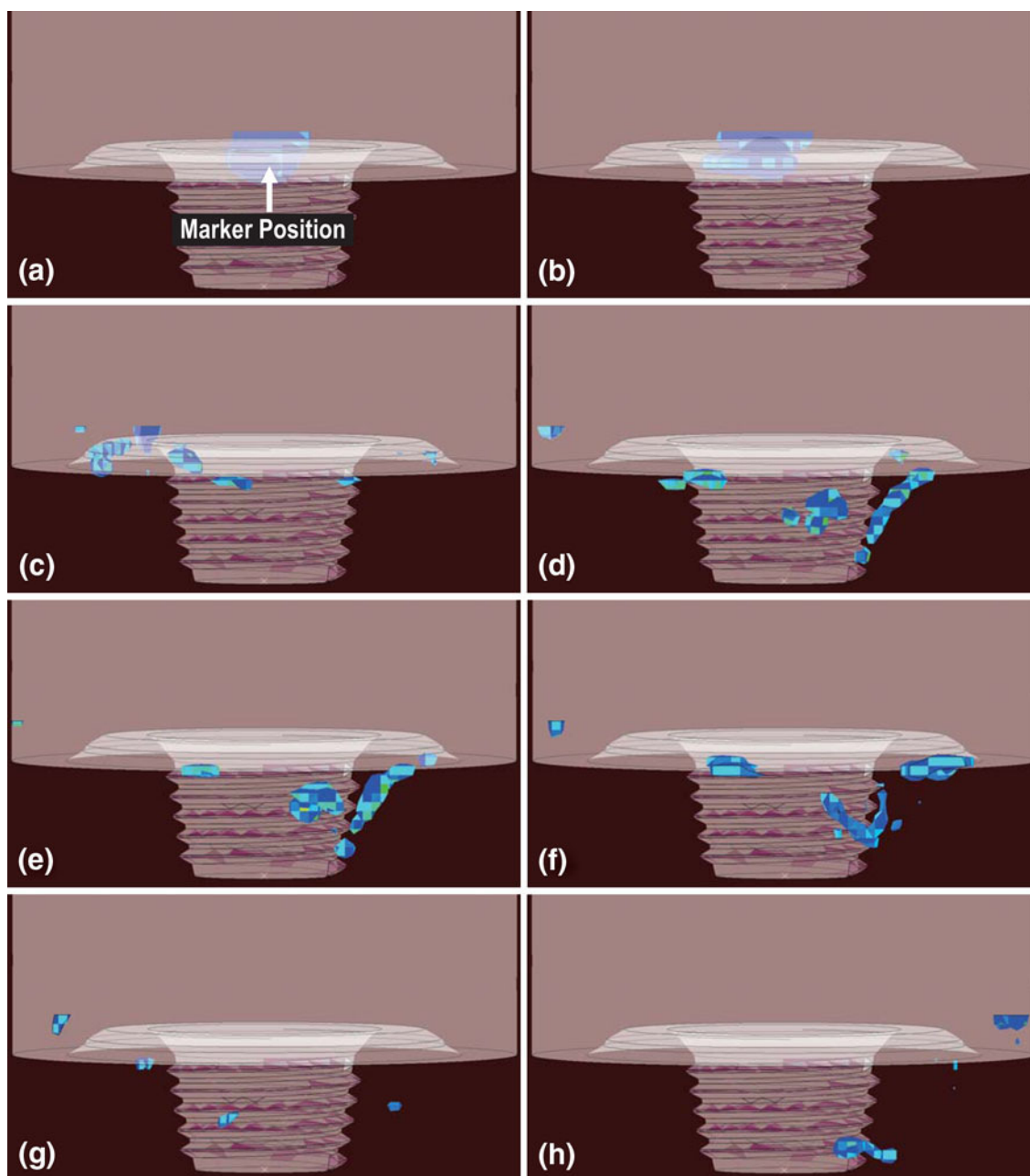
Fig. 10 Rear view of the spatial distribution and temporal evolution of the marker-material (initially located on the workpiece interface/top-layer) volume fraction (red greater than 0.8, blue less than 0.2): tool rotation speed = 500 rpm; tool travel speed = 0.0025 m/s; tool tilt angle = 2.5°; tool plunge depth = 0.0001 m; 10 mm upper-diameter tool pin; welding time in seconds: (a) 2.7, (b) 6.6, (c) 10.5, (d) 14.4, (e) 18.3, (f) 22.2, (g) 26.1, (h) 30
