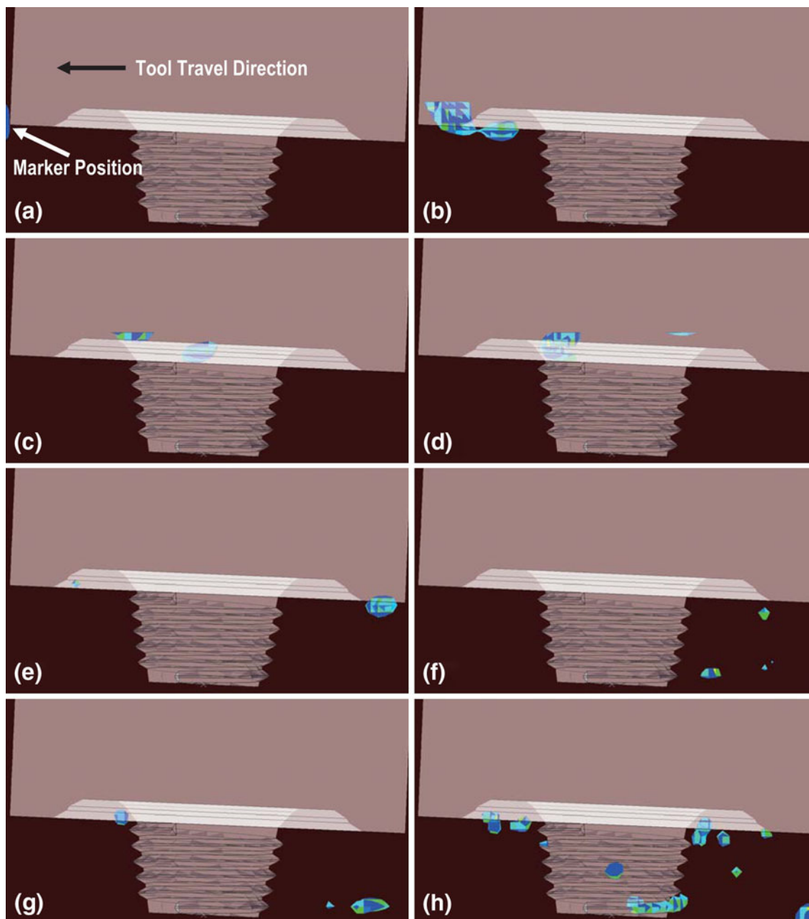
Fig. 5 Side view of the spatial distribution and temporal evolution of the marker-material (initially located on the workpiece advancing-side/top-layer) volume fraction (red greater than 0.8, blue less than 0.2); tool rotation speed = 500 rpm; tool travel speed = 0.0025 m/s; tool tilt angle = 2.5°; tool plunge depth = 0.0001 m; 10 mm upper-diameter tool pin; welding time in seconds: (a) 2.7, (b) 6.6, (c) 10.5, (d) 14.4, (e) 18.3, (f) 22.2, (g) 26.1, (h) 30
