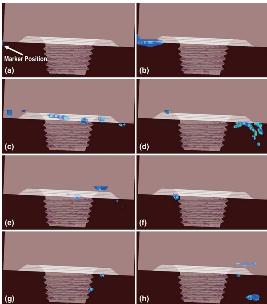
Fig. 8 Side view of the spatial distribution and temporal evolution of the marker-material (initially located on the workpiece interface/top-layer) volume fraction (red greater than 0.8, blue less than 0.2); tool rotation speed = 500 rpm; tool travel speed = 0.0025 m/s; tool tilt angle = 2.5°; tool plunge depth = 0.0001 m; 10 mm upper-diameter tool pin; welding time in seconds: (a) 2.7, (b) 6.6, (c) 10.5, (d) 14.4, (e) 18.3, (f) 22.2, (g) 26.1, (h) 30
