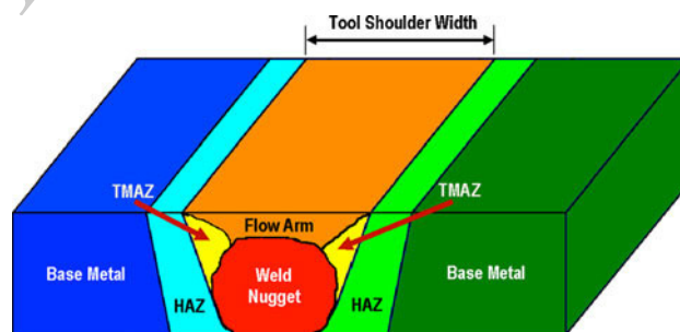
Fig. 3 A schematic of the main microstructural zones associated with the typical FSW joint
