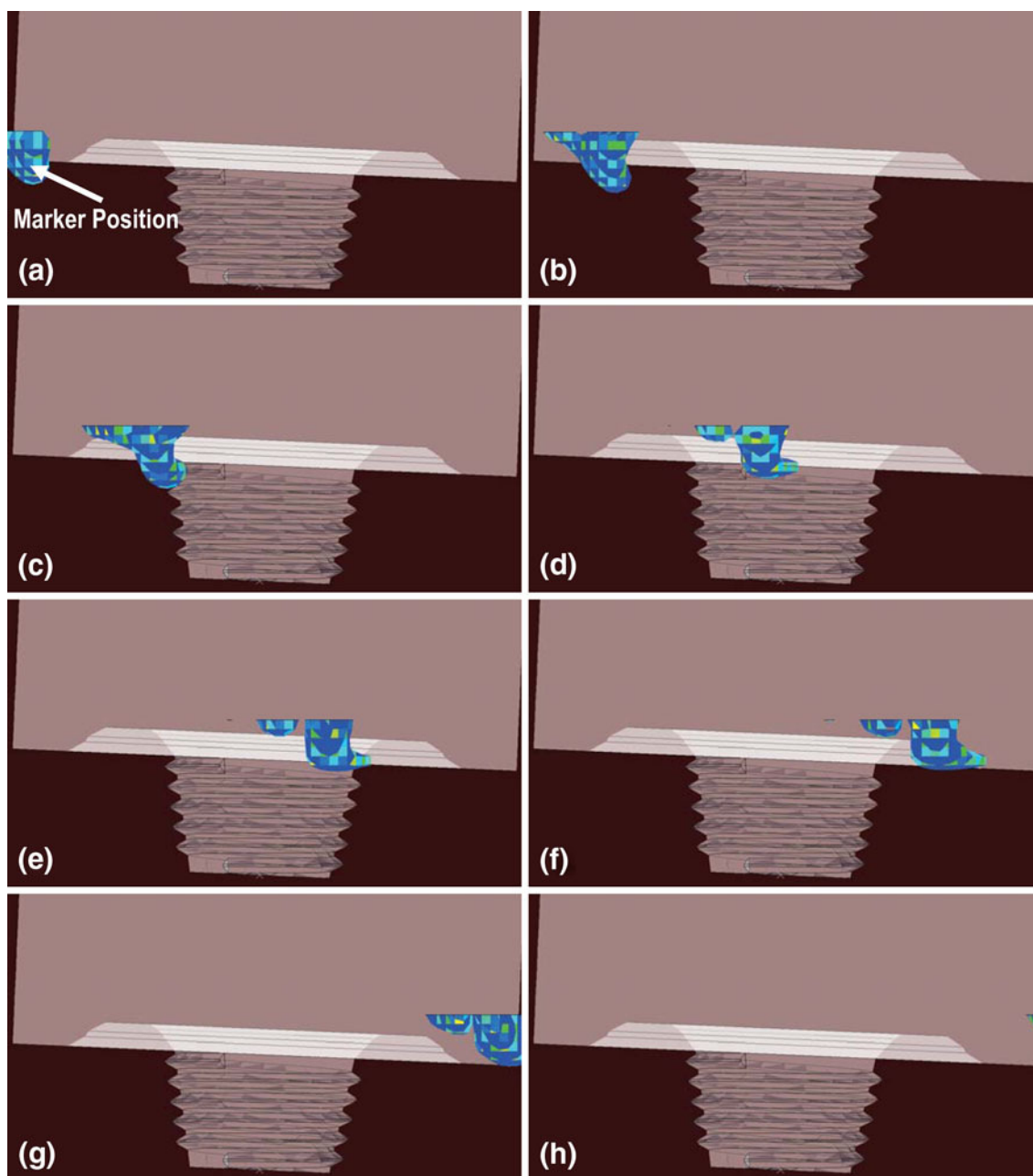
Fig. 11 Side view of the spatial distribution and temporal evolution of the marker-material (initially located on the workpiece retreating side/top-layer) volume fraction (red greater than 0.8, blue less than 0.2): tool rotation speed = 500 rpm; tool travel speed = 0.0025 m/s; tool tilt angle = 2.5°; tool plunge depth = 0.0001 m; 10 mm upper-diameter tool pin; welding time in seconds: (a) 3.9, (b) 5.4, (c) 7.2, (d) 8.4, (e) 9.9, (f) 11.4, (g) 12.9, (h) 14.4
