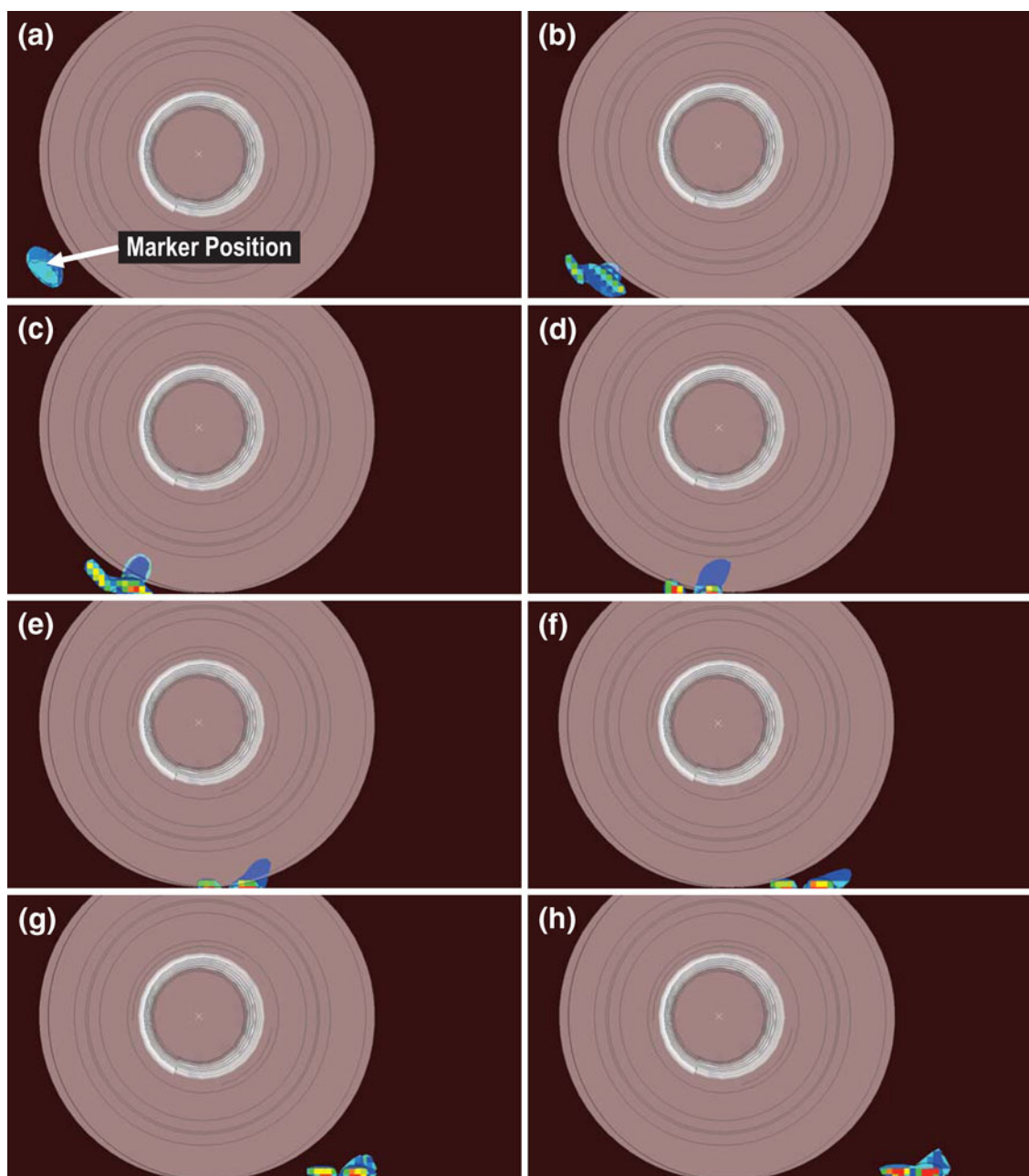
Fig. 12 Top view of the spatial distribution and temporal evolution of the marker-material (initially located on the workpiece retreating side/top-layer) volume fraction (red greater than 0.8, blue less than 0.2): tool rotation speed = 500 rpm; tool travel speed = 0.0025 m/s; tool tilt angle = 2.5°; tool plunge depth = 0.0001 m; 10 mm upper-diameter tool pin; welding time in seconds: (a) 3.9, (b) 5.4, (c) 7.2, (d) 8.4, (e) 9.9, (f) 11.4, (g) 12.9, (h) 14.4
