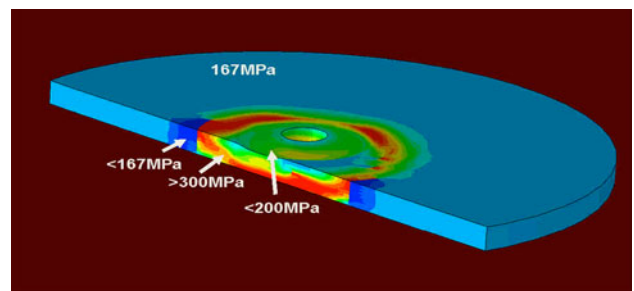
Fig. 11 An example of the spatial distribution of room-temperature material yield strength across a transverse section of a FSW joint in AA5083-H131. Material initial yield strength is 167 MPa
