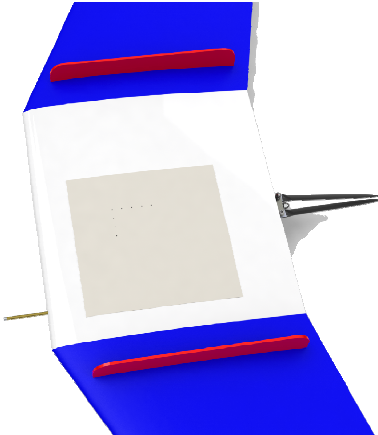
Figure 4. Embedded acoustic array in center section
