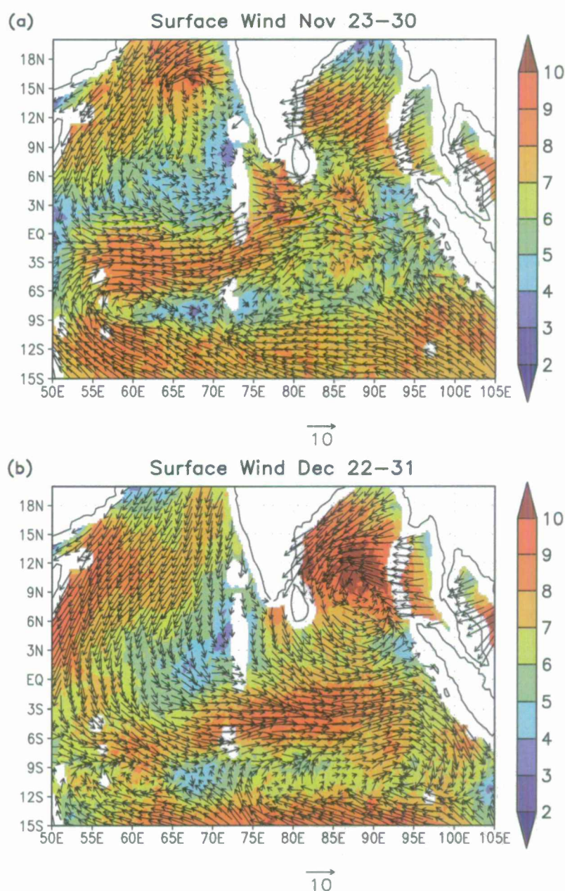
Figure 3. (a) Average winds (m/s) at 10 m (arrows) and wind speed (shading) from Windsat during 23–30 November 2011. (b) Same as (a) except the periods 22–31 December 2011.
