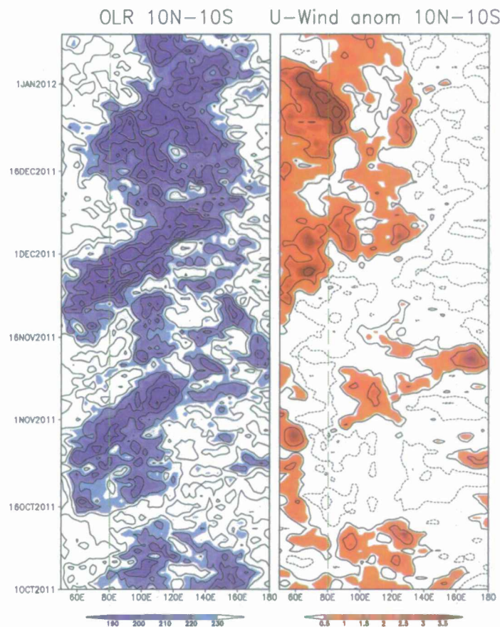
Figure 1. (Left): A longitude-time diagram of Outgoing Longwave Radiation (OLR) [14] averaged over 10°N–10°S. The dashed line (at 80°E) indicates the location of CINDY/DYNAMO ocean observations. (Right): Same as the left panel except for the surface zonal wind anomaly derived from the NCEP/NCAR reanalysis [15]. The anomaly is calculated by subtracting the annual cycle for the period 1979–2011.
