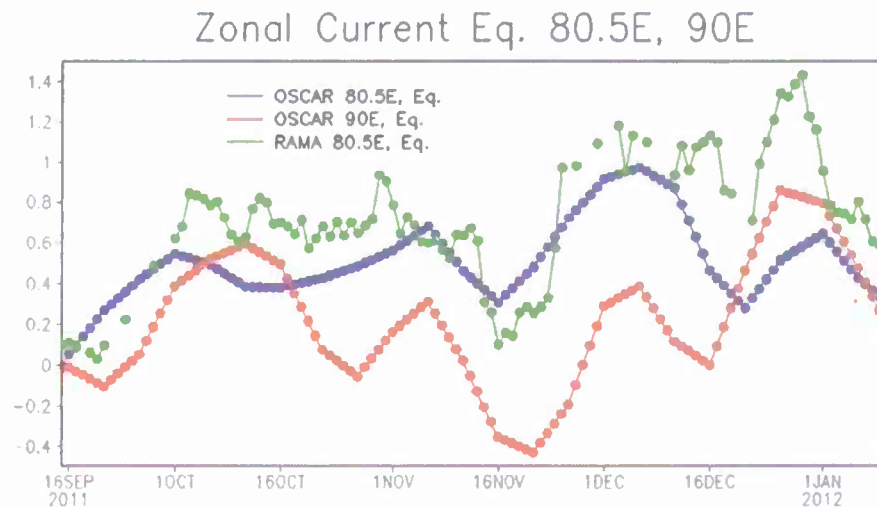
Figure 4. Zonal current (m/s) at 10 m at 80.5°E, equator (blue line) and 90°E, equator (red line) from OSCAR, and at 80.5°E, equator from the RAMA buoy (green line).
