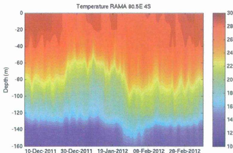
Figure 10. Time series of temperature ( ^{\circ}\text{C} ) profile from the RAMA buoy at 4^{\circ}\text{S} , 80.5^{\circ}\text{E} .
