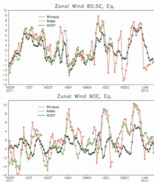
Figure 2. (Upper): 3-day average zonal winds (m/s) at 10 m height at 80.5°E, equator from Windsat (red), RAMA buoy (green), and the NCEP/NCAR reanalysis (black). (Lower): Same as upper panel except at 90°E, equator.
