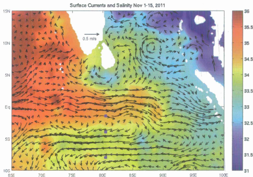
Figure 12. Average SSS (psu) derived from Aquarius measurements and near surface currents (m/s) from OSCAR during 1–15 November. RAMA buoy locations along 80.5°E are indicated by blue closed square marks. SSS data are interpolated to 0.2^\circ \times 0.2^\circ grid.
