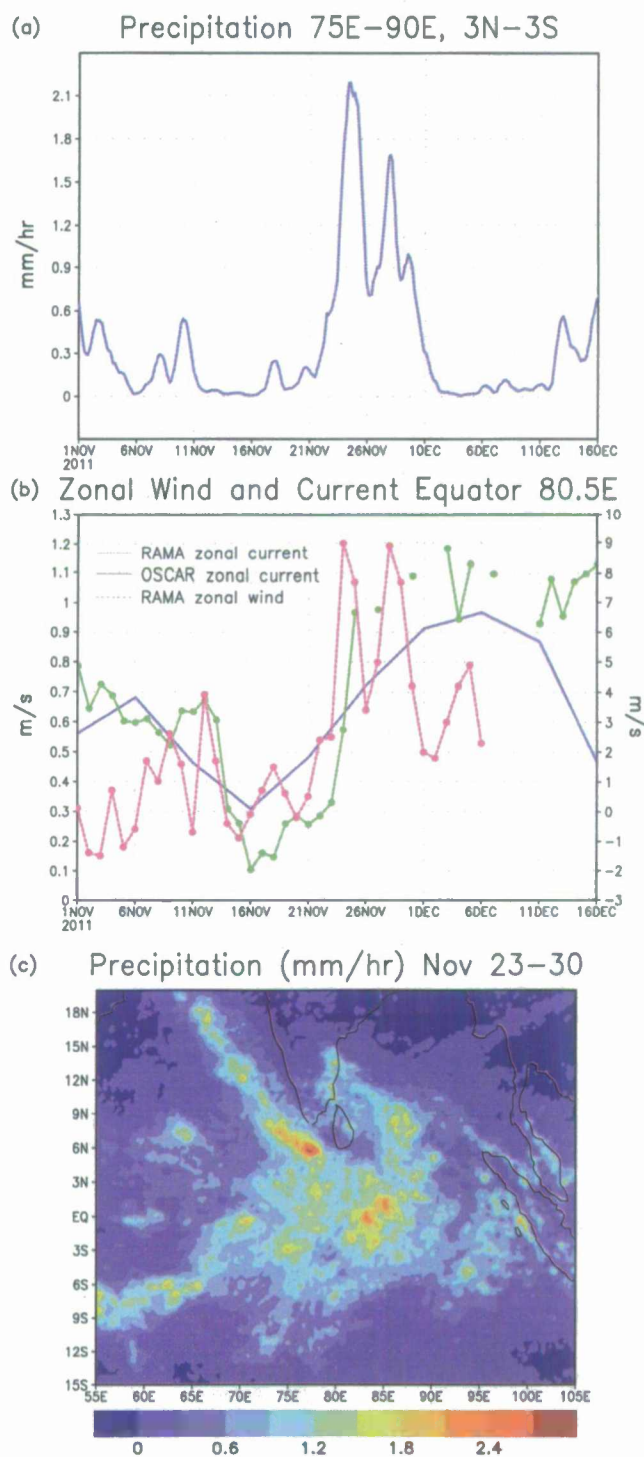
Figure 13. (a) Time series of precipitation averaged over 75°E–90°E, 3°N–3°S. (b) Time series of zonal wind and current at Equator, 80.5°E. Green lines indicate zonal current at 10 m depth from the RAMA buoy, and blue lines indicate near surface zonal current from OSCAR. Red dashed lines indicate zonal winds at 4m height measured by the RAMA buoy. (c) Average precipitation from TRMM 3B42 during 23–30 November 2011.
