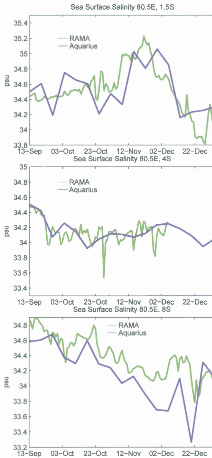
Figure 11. Time series of sea surface salinity (psu) in boreal fall 2011 estimated from Aquarius (blue line) and RAMA buoy (green line) at 80.5°E, 1.5°S ( top ), 80.5°E, 4°S ( middle ), and 80.5°E, 8°S ( bottom ).
