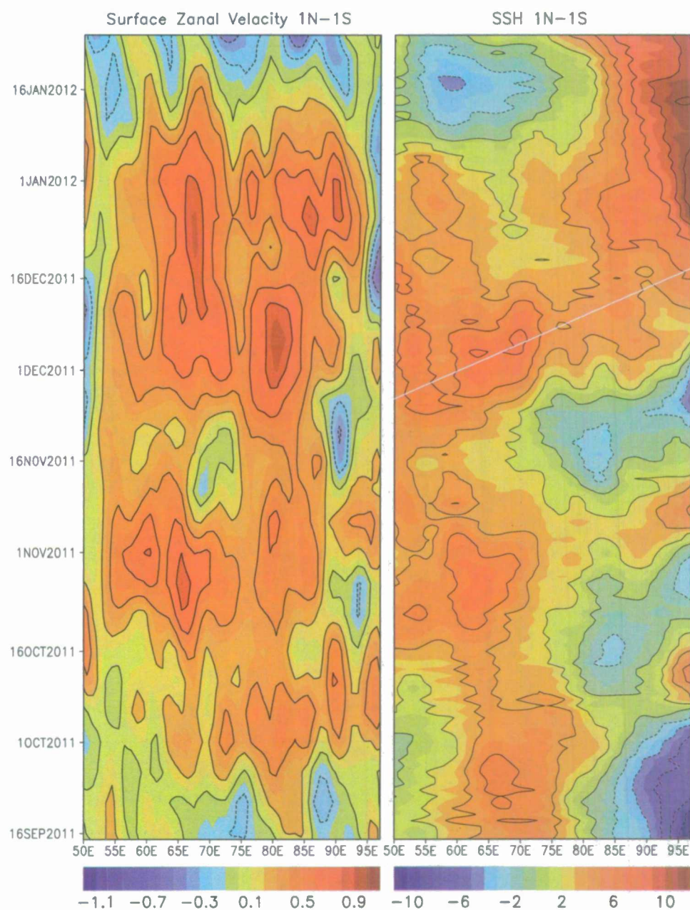
Figure 5. (Left): Longitude-time diagram of near surface zonal velocity (m/s) averaged over 1^{\circ}\text{N} – 1^{\circ}\text{S} from OSCAR. (Right) Same as left panel except for sea surface height (SSH) anomaly (cm) derived from altimeter measurements. The white line indicates the phase speed of 2.8 m/s.
