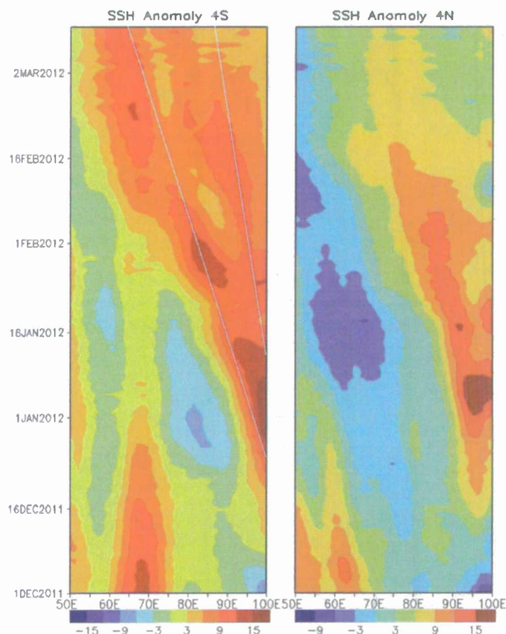
Figure 9. Longitude-time diagram of SSH anomaly (cm) at 4°S (left) and 4°N (right). The white lines indicate the phase speed of -0.66 m/s and -0.33 m/s.
