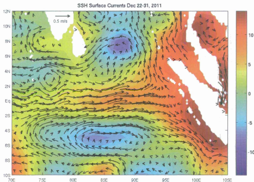
Figure 6. Average SSH anomaly (cm; shading) from altimetry and surface currents (m/s; arrows) from OSCAR during 22–31 December 2011.
