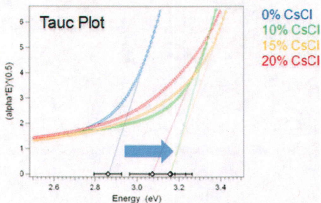
Fig.1 : Addition of CsCl to GNS glass blue-shifts the band edge by \sim 0.25 eV and enhances the Ce 3+ photoluminescence quantum yield.
