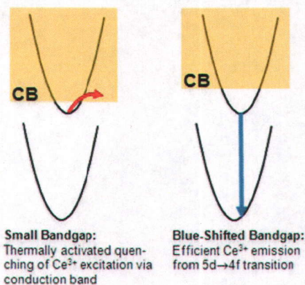
Fig. 2: Effect of conduction band edge position on the relaxation dynamics of the Ce 3+ excited state.
