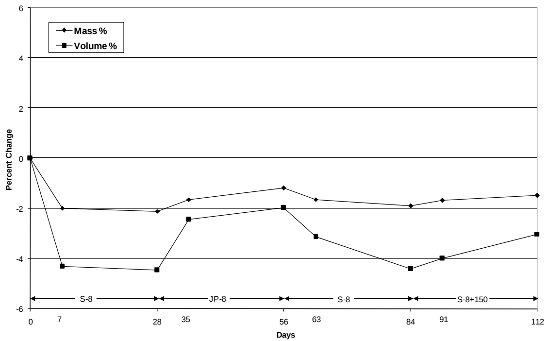
Stanadyne Pump New Transfer Pump Viton 0-Ring in Fuel Nf-2
