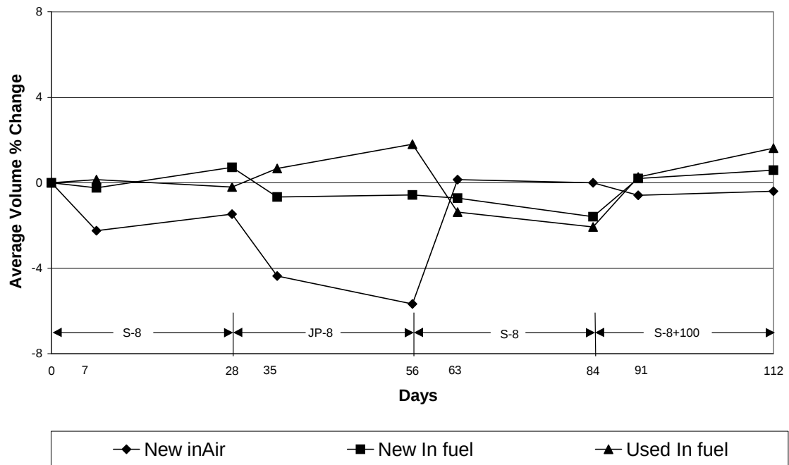
Detroit Diesel Unit Injector Viton Elastomers Volume Changes In Fuel
