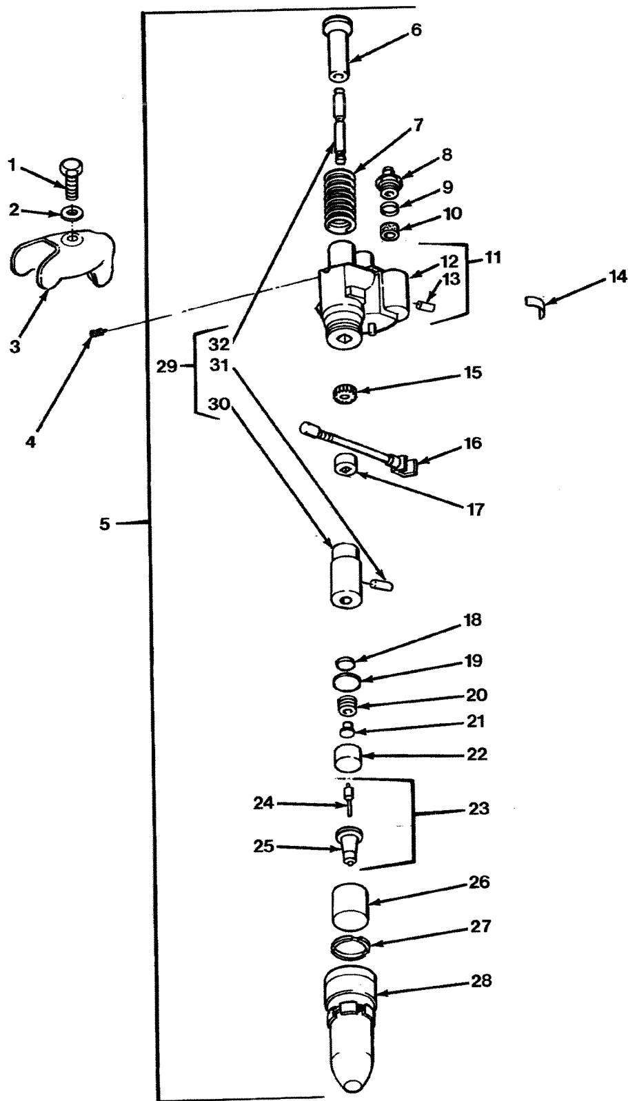
FIG.29 FUEL INJECTOR
