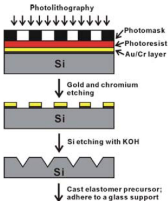
Figure 18. Schematic diagram of the polymer pen array fabrication process.
