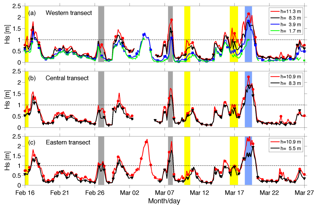
Figure 3. Significant wave height versus time across (a) the western transect in 11.3- (pv2, red curve), 8.3- (pv4, black), 3.9- (n15, blue), and 1.7-m (n4, green) water depths, (b) the central transect in 10.9- (pv7, red) and 8.3-m (pv9, black) water depths, and (c) the eastern transect in 10.9- (dw12, red) and 5.5-m (pv16, black) water depths. The dashed black lines at 1m height are for reference. Data gaps for shelf stations between March 2 and March 5 are due to instrument maintenance. Shaded areas refer to events discussed in the text and indicate periods with large spatial wave variability and strong ( > 9 m/s) winds from the northeast (yellow, 0 < \text{dir} < 80 deg) and northwest (gray, 300 < \text{dir} < 360 deg), as well as a period of large swell (blue).
