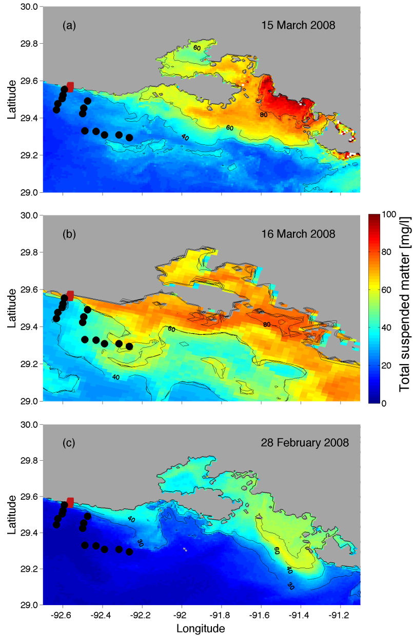
Figure 5. Estimate of total suspended-matter concentrations (from Modis 250 imagery) on (a) March 15, (b) March 16, and (c) February 28. All images were recorded around 17:00 o'clock GMT. High concentrations are red, low concentrations are blue (color scale on right). Grey shading is land. Instrument locations are shown with black circles (shelf stations) and red squares (shoreward stations).
