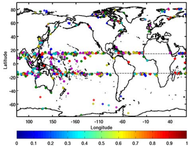
Figure 7: Significant bicoherence values at each grid location from the baroclinic velocities in layer 14 (laying at about 500 m over much of the ocean) from HYCOM. Only locations at which the subharmonic energy is at least 1% of the primary waves are shown.
