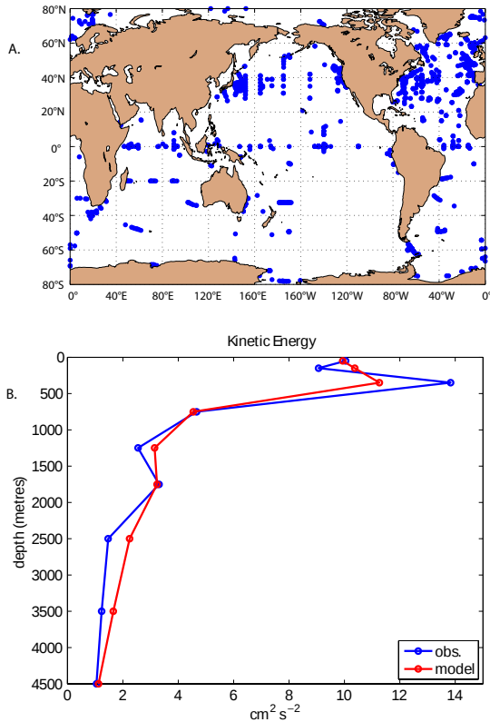
Figure 5: (a) Horizontal locations of current meters used to validate the tidal currents in the HYCOM simulations. Units of x- and y-axes are degrees. (b) Vertical distributions of the M_2 tidal
