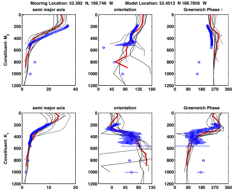
Figure 4: Vertical structure of tidal currents in ADCP data at a particular North Pacific location (blue curves), nearest model gridpoint in HYCOM (red curves), and in eight surrounding model gridpoints (black curves). Top/bottom panels are for M_2 / K_1 , respectively. Left/middle/right panels show semi-major axis, orientation, and Greenwich phase, respectively.
