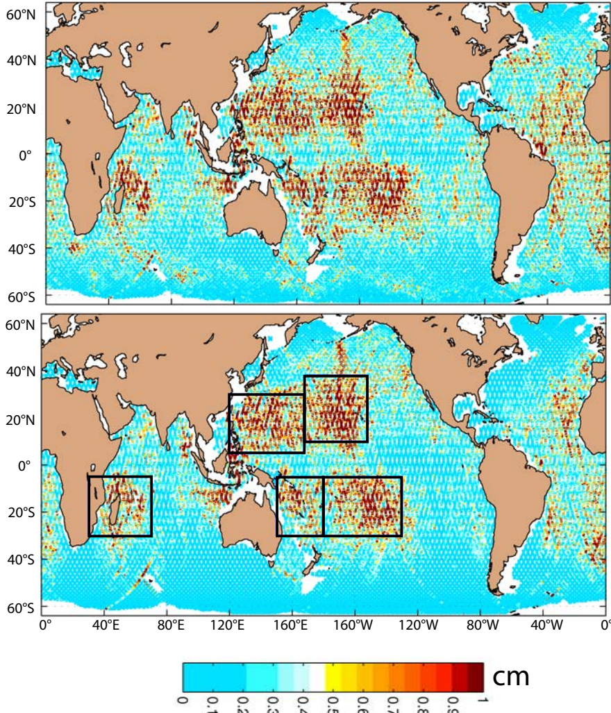
Figure 1: Amplitude (cm) of M_2 internal tide signature in sea surface height, obtained from high-passing the M_2 amplitudes of the full sea surface height. Upper panel: results from satellite altimetry. Lower panel: results from HYCOM.
