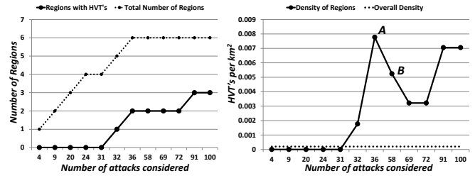
Figure 3: Number of attacks vs. number of regions and HVT density.
