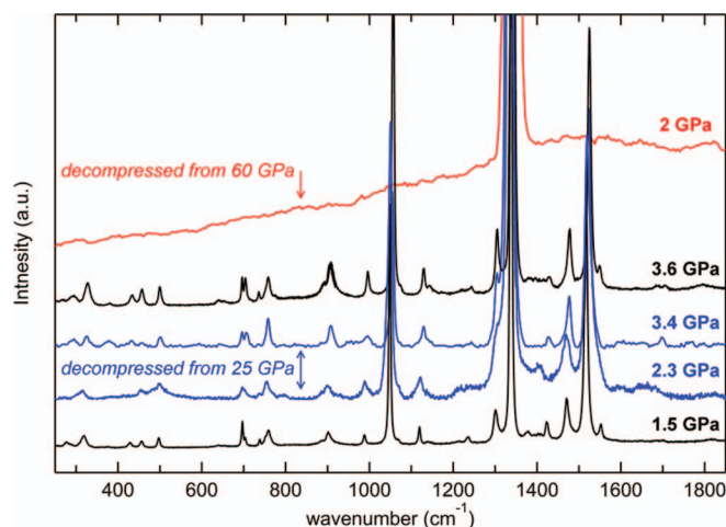
FIG. 11. Comparison of Raman measurements taken on compression (black) with those obtained on decompression. Data from samples decompressed from 25 \text{ GPa} and 60 \text{ GPa} are blue and red, respectively; blue curves correspond to samples loaded hydrostatically (upper) and nonhydrostatically (lower). Excitation wavelengths from top to bottom are 488 , 488 , 632 , 457 , and 488 \text{ nm} .
