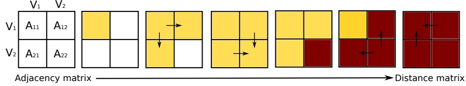
Fig. 2. DC-APSP algorithm, with initial adjacency distance denoted in white, partially complete path distances in yellow, and final path distances in red
