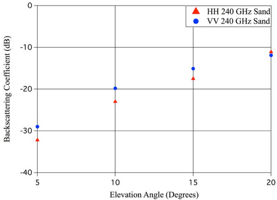
Figure 16: HH and VV polarized backscattering coefficients for sand at 240 GHz.
