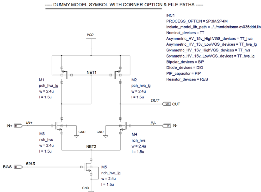
Figure 3 Differential Amplifier Used in CTIA and Output Sample Buffer
