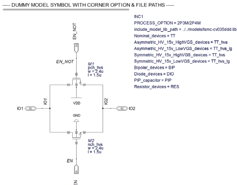
Figure 4 Transfer Gates Used to Switch Analog Signals
