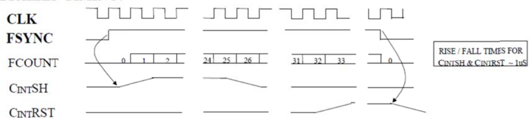
Figure 17 - FSYNC Timing Details
