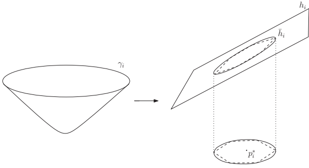
Figure 5. In the case of the Euclidian metric, \gamma_i can be simplified using the lifting transform.
