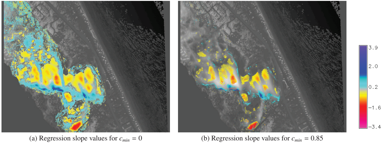
Figure 7. Regression line slope values from year 2000 to 2006 superimposed on year 2000 DEM.
