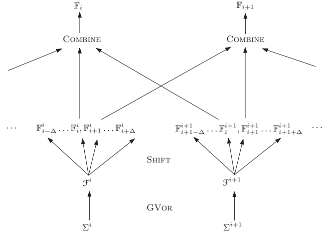
Figure 6. The process of creating \mathbb{F}_i from sets of data \Sigma^i rendering each point only once.
