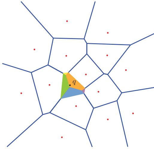
Figure 2. Natural neighbor interpolation for a point set S and query point q in \mathbb{R}^2 . The shaded cell is \text{Vor}_{S \cup \{q\}}(q) , and each color denotes the area stolen from each cell of \text{Vor}(S) .
