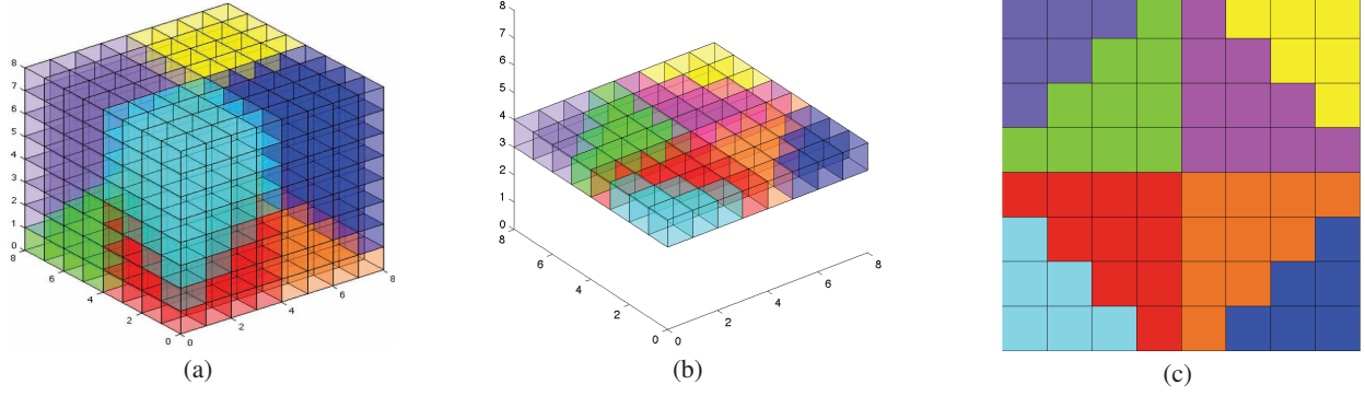
Figure 3. Pixelized Voronoi Diagram where d(\cdot, \cdot) is the Euclidean metric. (a) \text{PVor}(S) for a set of eight points; (b,c) \text{PVor}_S(3) , shown as a slice of \mathbb{B} from (a).
