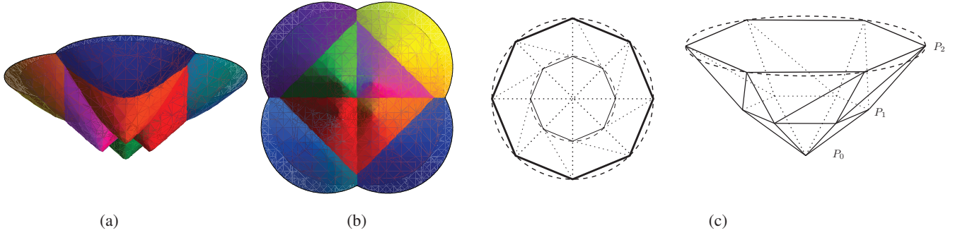
Figure 4. (a,b) Lower envelope of 8 points that were used for \text{PVor}(S) in Figure 3(b,c). (a) shows the hyperboloids from a side view; (b) the outer cells of the Voronoi diagram are infinite, but in this figure their sizes are limited because the hyperboloids are of a limited height. (c) The triangulation of \gamma_i into \gamma_i^\circ using two triangle strips ( m = 2 ).
