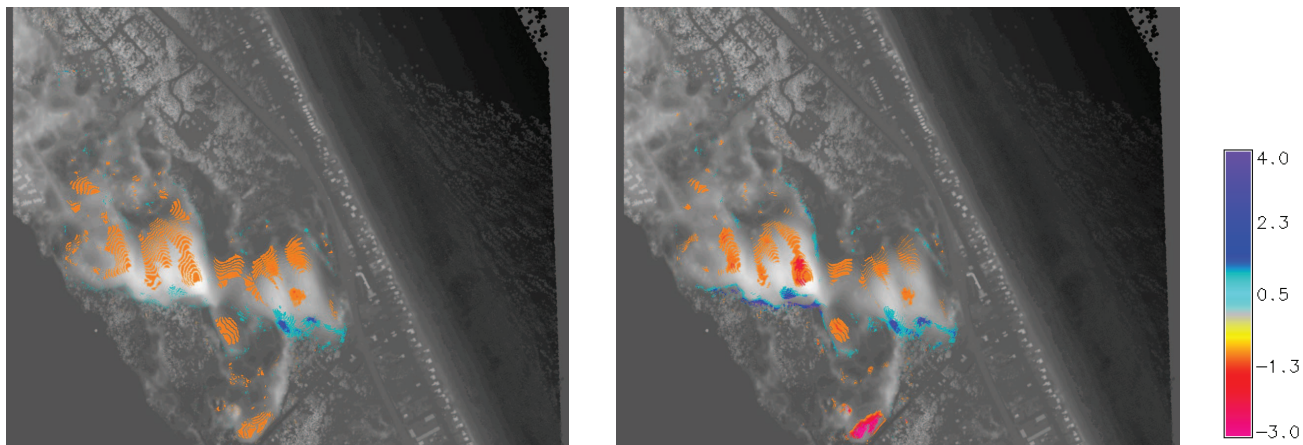
(a) Changes from 2002 to 2003 superimposed on 2002 DEM (b) Changes from 2003 to 2004 superimposed on 2003 DEM
