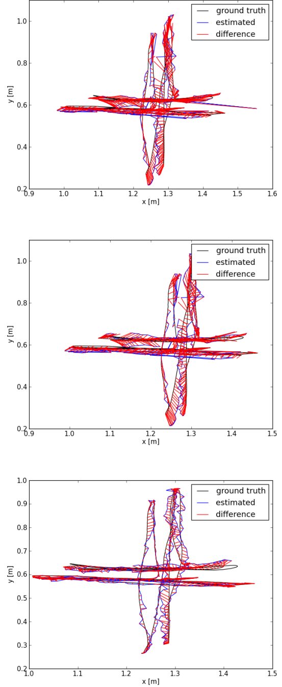
Figure 20: XYZ Absolute Trajectory Plots (RANSAC,Dynamic RGB-D,RGB-D SLAM)
