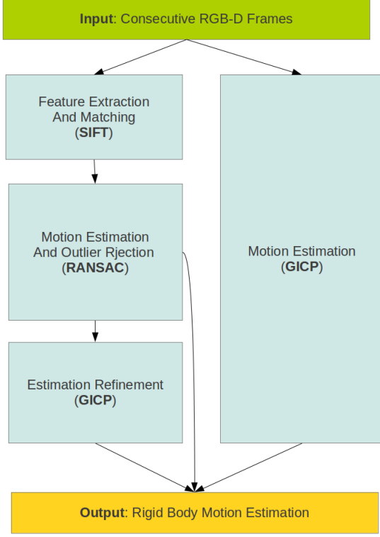
Figure 9: plane-to-plane algorithm flow
