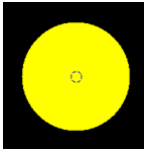
Figure 15. Zoom-out task.
