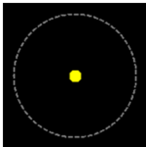
Figure 14. Zoom-in task.
