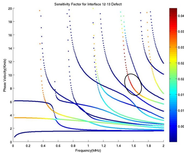
Figure 3.44. Sensitivity factor of semi-shear horizontal waves on a dispersion curve for detecting delaminations between layers 12 and 13. Wave launching direction is 0 degree. The region circled indicates good loading function choices for delamination along interface 12-13.
