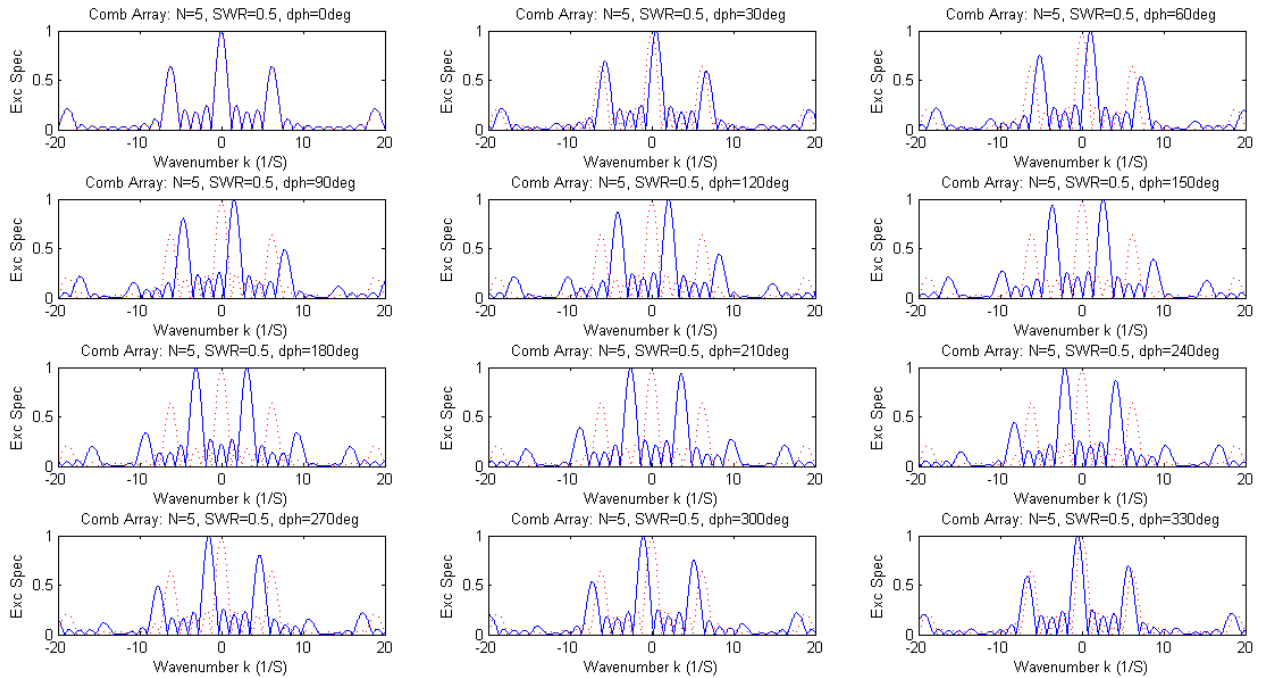
Fig. 25 Excitation spectrum of linearly-phased 5-element comb array in k -domain.
