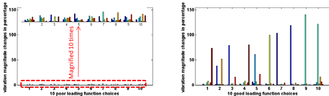
Figure 8.30. Vibration magnitude changes in percentage from 50% torque reduction on bolt 10 to bolt 10 removal, under (Left) 10 poor loading function choices and (right) 10 good loading function choices, showing significant differences in vibration amplitude variations due to different loading function choices..
