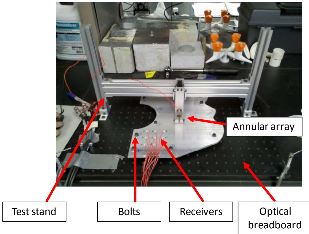
Figure 8.22. Experimental setup
