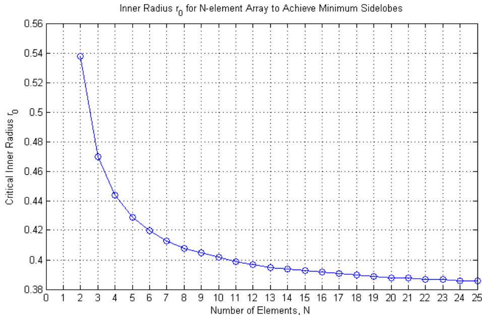
Fig. 2.10 The critical inner radius, r_c , for which the amplitudes of the subpeaks are minimized (and equal), can be found for any number of elements in an annular array.
