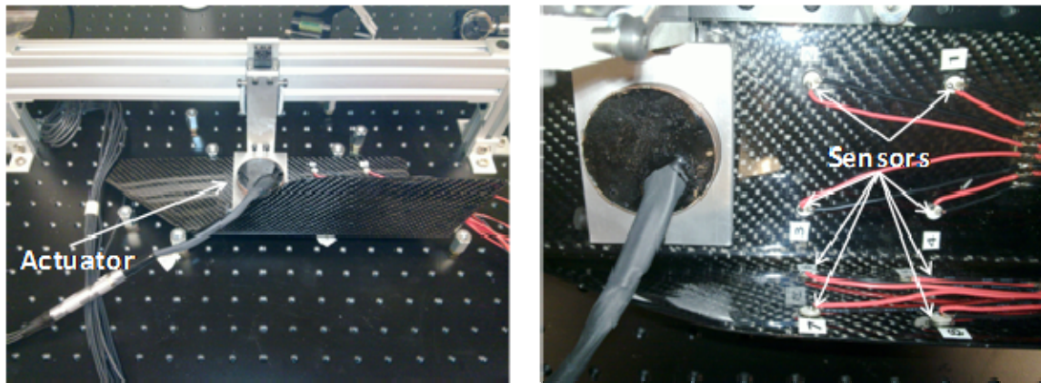
Figure 8.35. Experimental setup.
