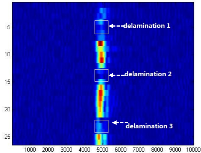
Figure 7.4 Guided wave scan image using mode 8 at 1.03MHz, showing good sensitivity to all three defects. It appeared that the decrease in amplitude was the least for the delamination defect 3 and the most for the center delamination which agreed with the sensitivity calculation results:
