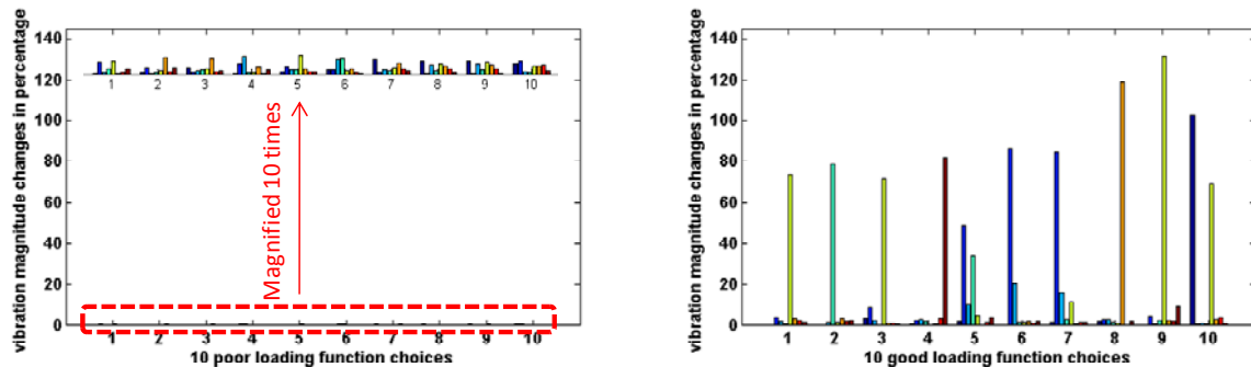
Figure 8.31. Vibration magnitude changes in percentage due to the introduction of a 30% depth corrosion, under (Left) 10 poor loading function choices and (right) 10 good loading function choices, showing significant differences in vibration amplitude variations due to different loading function choices.
