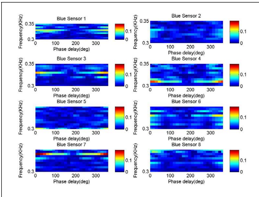
Figure 8.27. Amplitude map comparison between Test VII and Test I.
