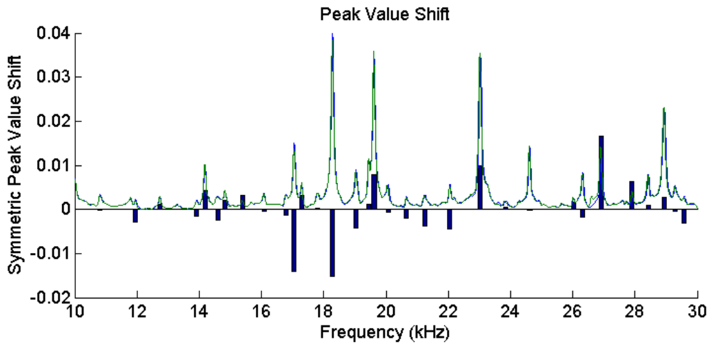
Fig. 8.12 The healthy spectrum (blue line), notch damage spectrum (green line), and shift in peak values (bars) for symmetric excitation.
