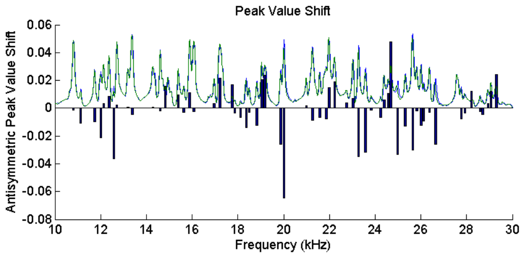
Fig. 8.13 The healthy spectrum (blue line), notch damage spectrum (green line), and shift in peak values (bars) for antisymmetric excitation.
