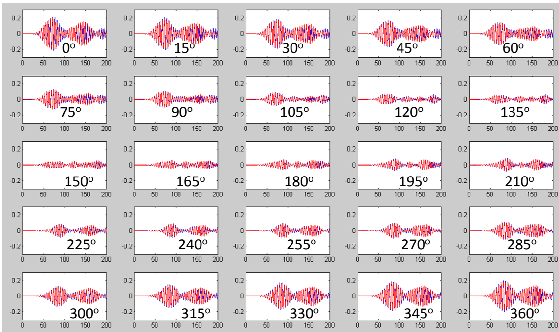
Figure 8.46. Transient guided wave signals for 200 kHz tone burst inputs with different phase delays applied to the four elements of the annular array actuator.
