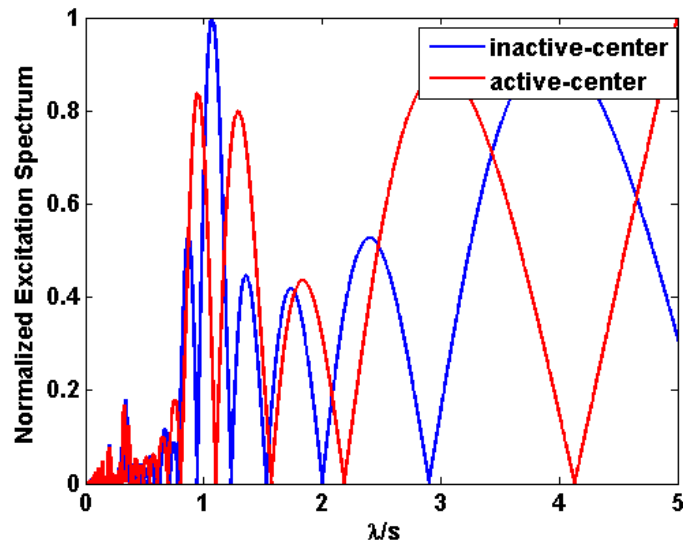
Fig. 2.5 Comparison between an inactive-center array and an active-center array; for the inactive-center array, r_0=2 mm. Number of elements N=3 elements, element width w=2 mm, and spacing s=4 mm.
