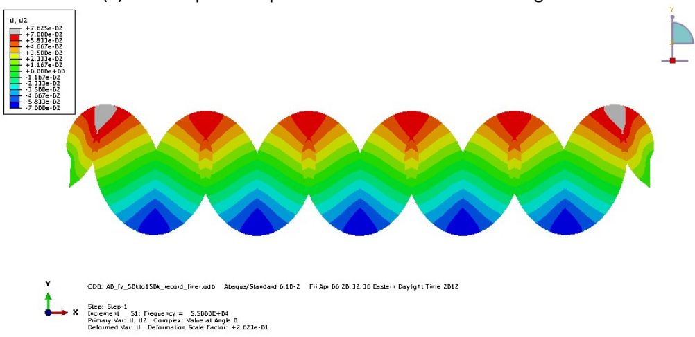
(b) Out-of-plane displacement field under A0 loading at 55000Hz
