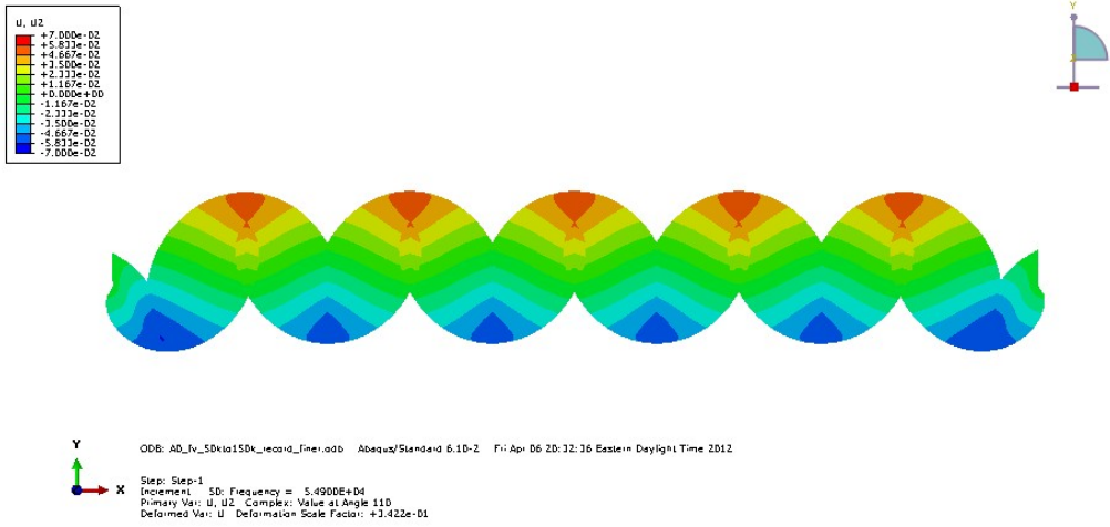
(a) Out-of-plane displacement field under A0 loading at 54900Hz
