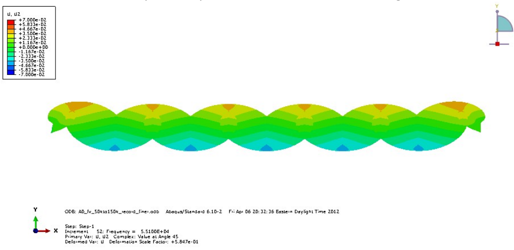
(c) Out-of-plane displacement field under A0 loading at 55100Hz
