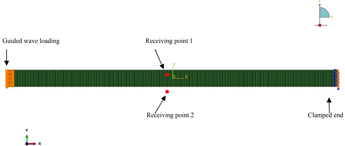
Figure 3.25. Model setup of forced vibration in ABAQUS
