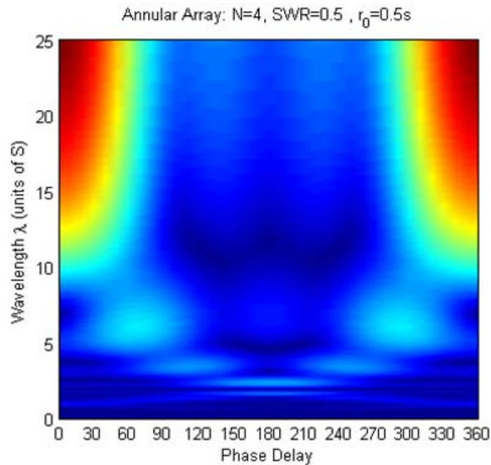
Fig. 2.41 Contour plot of excitation in the wavelength domain for a 4-element annular array over various phase delay values. Notice the poor selectivity in the upper region of \lambda > 10s .
