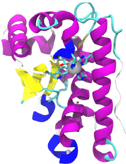
Figure 2. Ribbon representation of the E1-SOD model. The protein is colored by secondary structure elements (a-helix=purple, b-strand=yellow, 3-10 helix=blue, turn=cyan, coil=white ). Relevant residues of the Mn binding site are shown in licorice representation and colored by element (carbon=cyan, nitrogen=blue, oxygen=red). A representative Mn atom is displayed in vdW representation. Figure 3 made with VMD (Humphrey et al., 1996).
