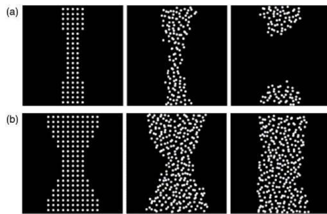
Figure 9. Snapshots of capillary dynamics of a liquid thread: L/D = 4.51 (top) and L/D = 2.5 (bottom).
