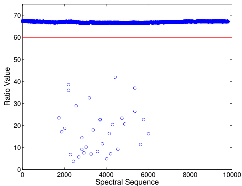
Figure 5.6. The ratio of intensities at 4570 \text{ cm}^{-1} and 4100 \text{ cm}^{-1} of all original single-beam spectra in Group 1. The red line shows the threshold value of 60 used to identify spectra altered by the presence of air bubbles.
