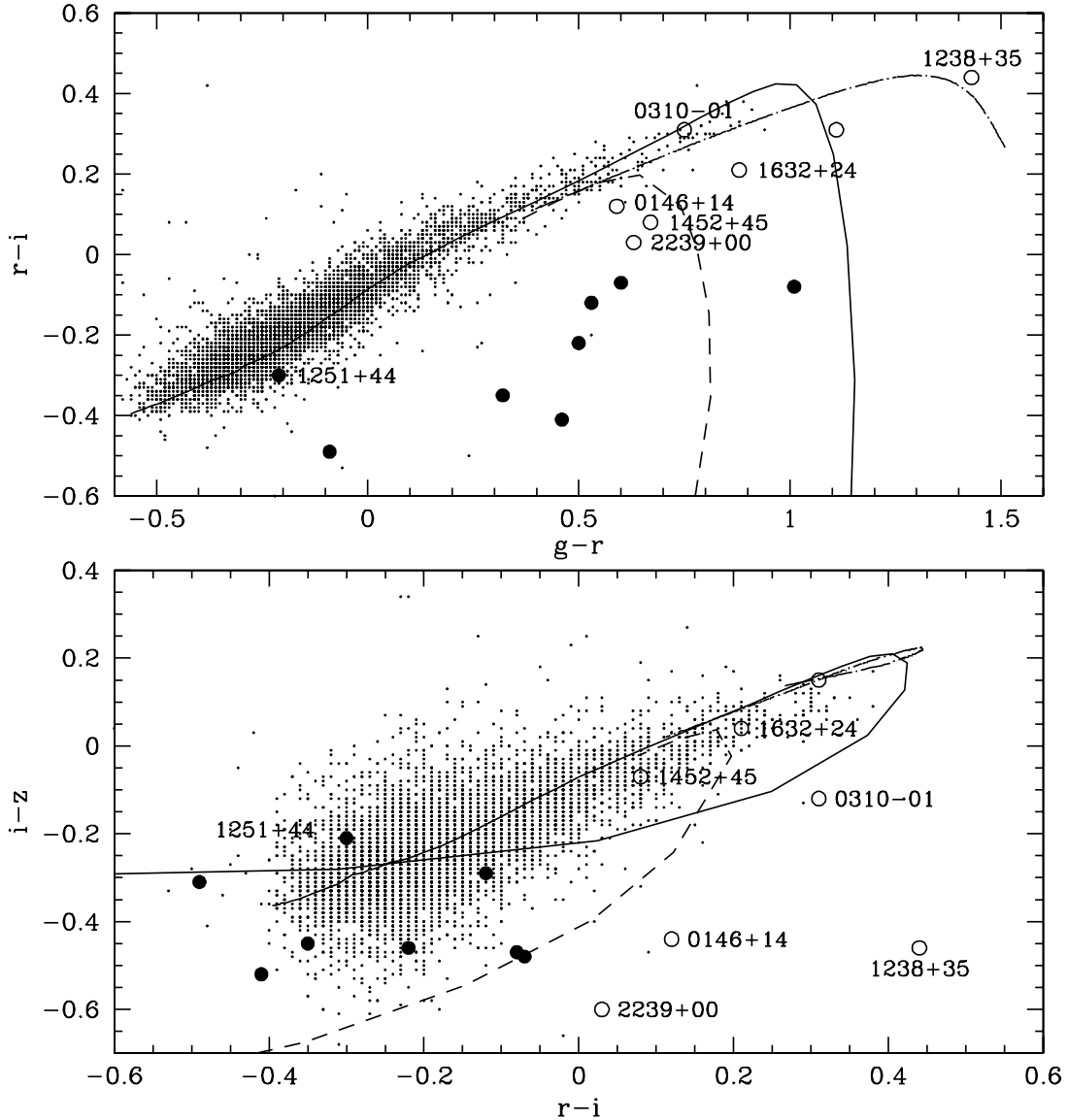
FIG. 2.—Color-color plots for ultracool white dwarfs in SDSS colors. Ultracool white dwarfs observed by SDSS are shown as filled circles for strong-CIA stars and open circles for mild-CIA stars. New stars identified in this paper are labeled. The proper-motion-selected white dwarfs used for the luminosity function by Harris et al. (2006) are shown as dots for comparison. The curves show models for white dwarfs with \log g = 8 with atmospheres of pure hydrogen (Bergeron et al. 1995b; solid line), pure hydrogen (Kowalski & Saumon 2006; dot-dashed line), and \text{He}/\text{H} = 10^5 (Bergeron & Leggett 2002; short-dashed line).
