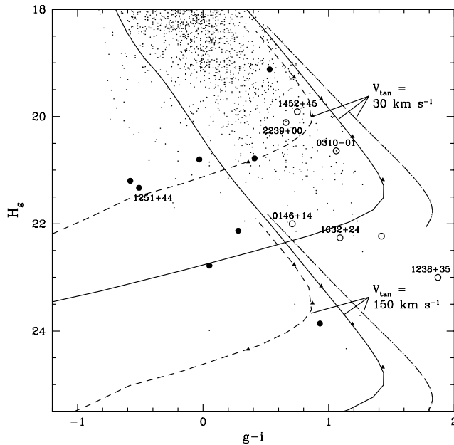
FIG. 3.— Reduced proper motion for ultracool white dwarfs observed by SDSS. The symbols and curves are the same as in Fig. 2. The model curves are plotted for two different assumed values of the tangential velocity, again assuming \log g = 8 . On each curve showing Bergeron models (solid line for hydrogen, short-dashed line for mixed composition), three triangles indicate ages of 6, 8, and 10 Gyr (top to bottom).
