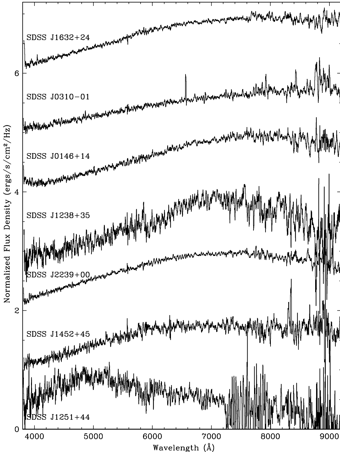
FIG. 1.—SDSS spectra for the seven new white dwarfs in this paper. Spectra have been smoothed by nine pixels to a resolution of 800, and are normalized and offset vertically by one unit for display. Compare with Fig. 2 of Gates et al. (2004) for SDSS spectra of previously observed cool white dwarfs.
