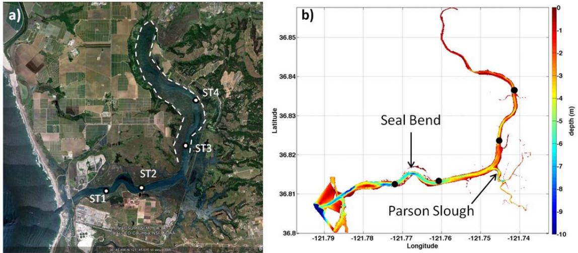
Figure 1. a) Google Earth image of Elkhorn Slough showing location of the 4 ADCP locations with white dots. The white dashed line highlights the low-lying marsh and mud flats at the shoreward end of the slough. b) 2011 bathymetry map of ES provided by CSUMB SFML. ADCP locations are shown with black dots. Depth color-scale provided on the right.
