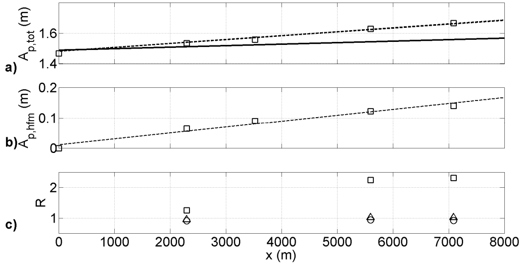
Figure 3. a) Squares represent A_{tot} between MB and ST4 as a function of along-channel distance. The dashed line is the best-fit line for A_{tot} estimated by linear regression. Solid line represents the Lamb (1932) analytical solution for co-oscillating tide for ES. b) A_{p,hfm} (squares) between MB and ST4 as a function of along-channel distance. The dashed line is the best-fit line for A_{p,hfm} estimated by linear regression. c) R_{tot} (triangles), R_{lfm} (circles), and R_{hfm} (squares) as a function of along-channel distance.
