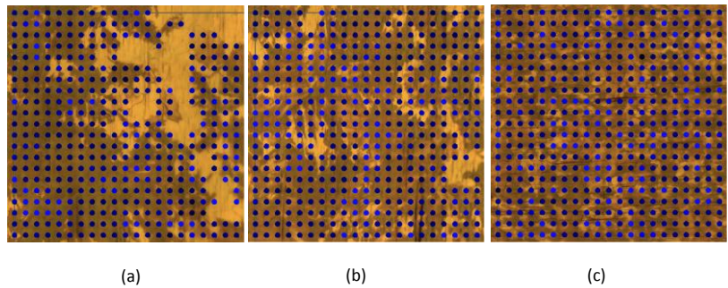
Fig. 3: Optical images of the surface of nickel substrates on which graphene has been grown at the temperatures of (a) 1000^\circ\text{C} , (b) 950^\circ\text{C} , and (c) 900^\circ\text{C} .
