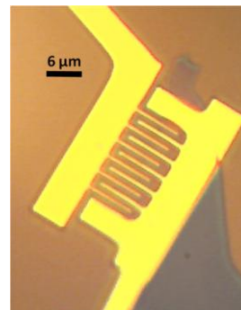
Fig. 4: Photomicrograph of a prototype metal-graphene-metal structure for investigating p-type and n-type doping in light sensing devices.
