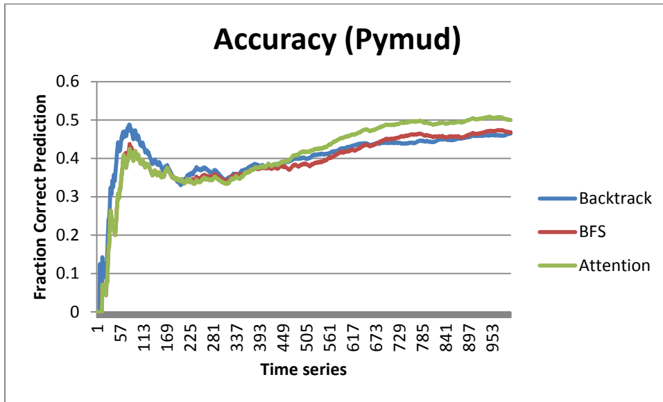
Figure 64. Pymud 1x1000: Prediction Accuracy.
