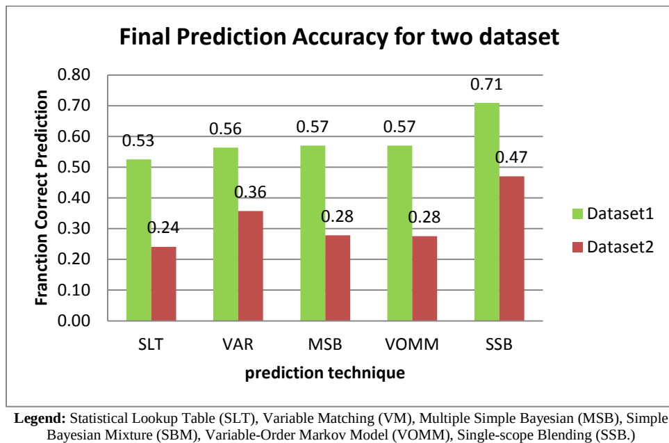
Figure 42. Final Prediction Accuracies for Dataset 1 and 2.
