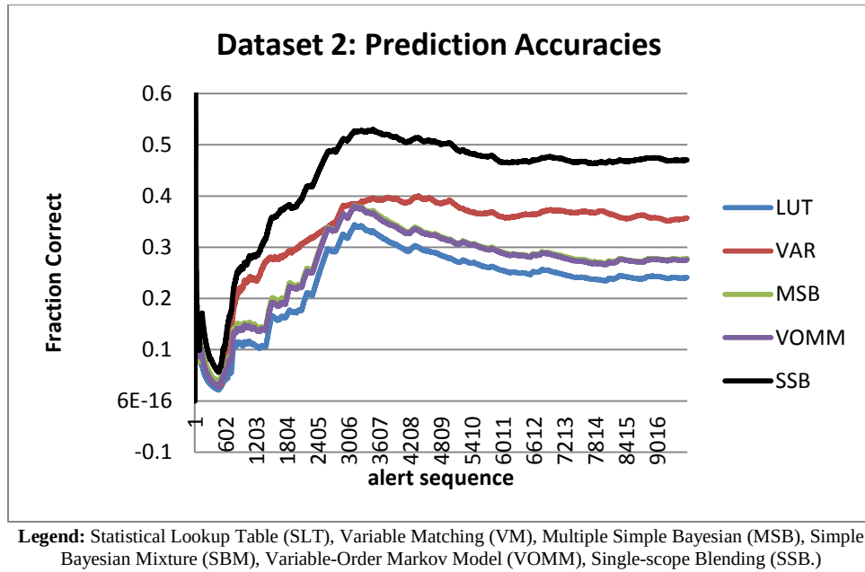
Figure 41. Dataset 2: Prediction Accuracy.
