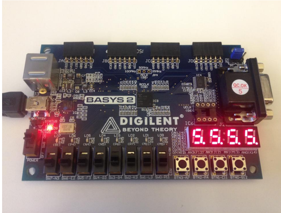
Figure 24. Digilent BASYS2 development board counting with proper state logic.
