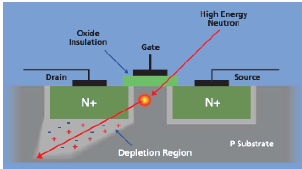
Figure 4. Neutron radiation strike of silicon atom resulting in ejection of heavy ions leading to firm error in transistor (From [21]).
