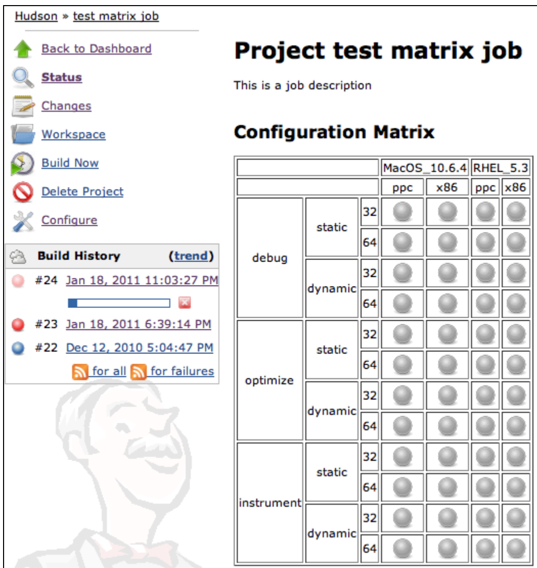
Figure 19. Continuous Build/Test Dashboard Configuration
