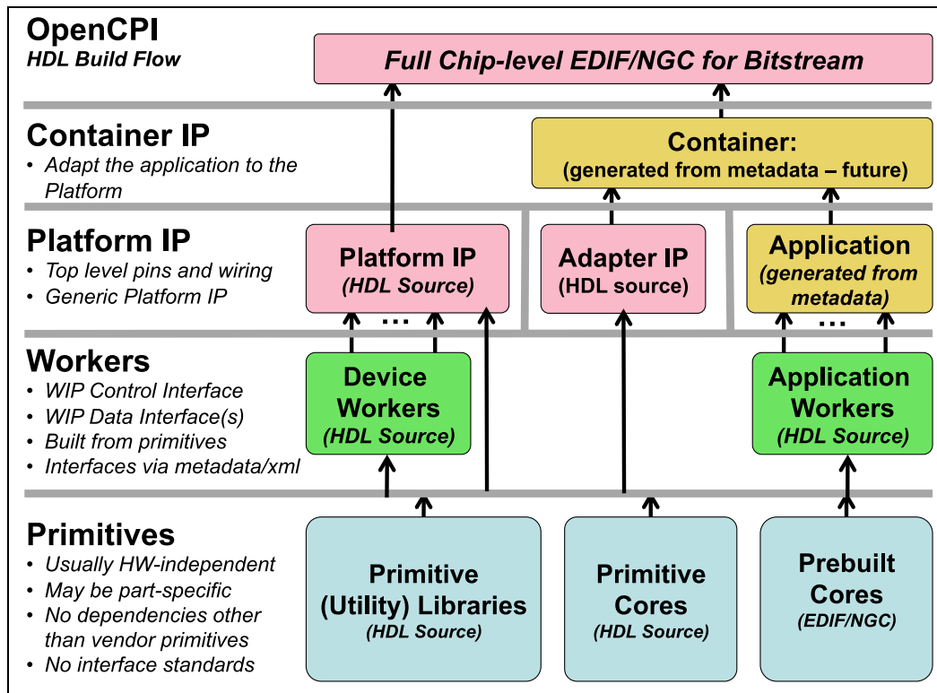
Figure 9. OpenCPI HDL Build Flow
