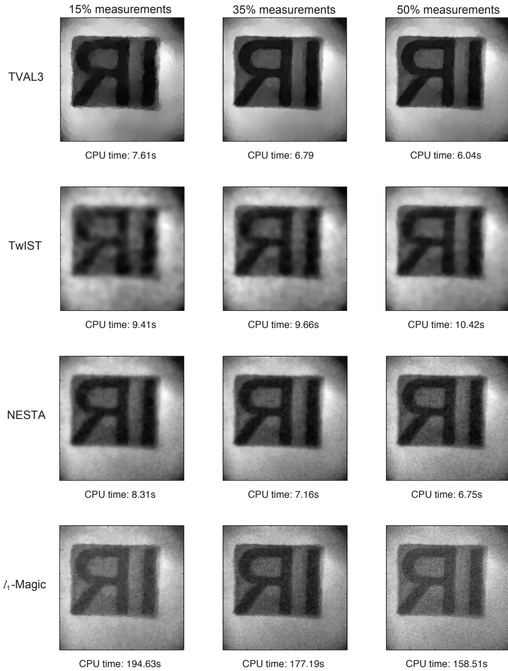
Figure 5: Recovery of a 256 \times 256 infrared image. The four rows (top to bottom) are reconstructed by TVAL3, TwIST, NESTA and \ell_1 -Magic, respectively, for sampling ratios (left to right) 15%, 35%, and 50%, respectively.
