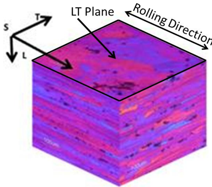
Figure 3. Orientation of L, T Directions and LT Plane with Respect to the Microstructure. From [7]
