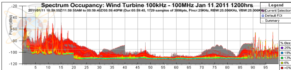
Figure 8. Ambient Spectrum Sample for 100 kHz to 100 MHz for 11 January 2011 (from Sasarita, 2013, p. 2-8)
