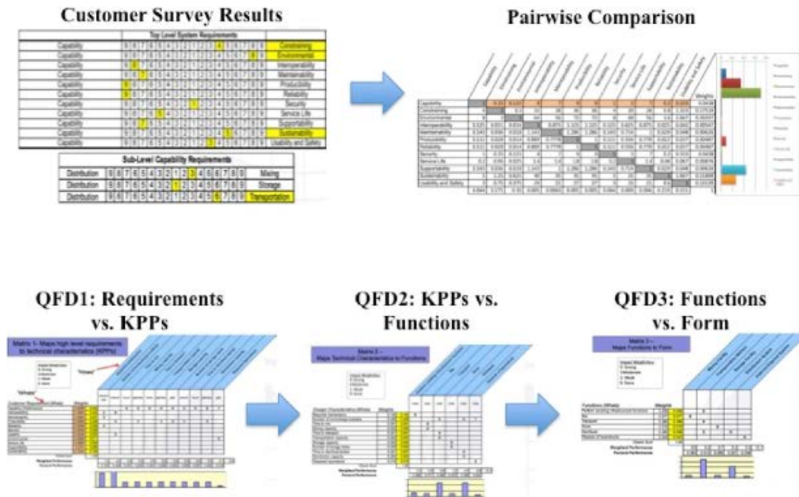
Figure 9. Value Modeling Process using AHP to Develop HOQ
