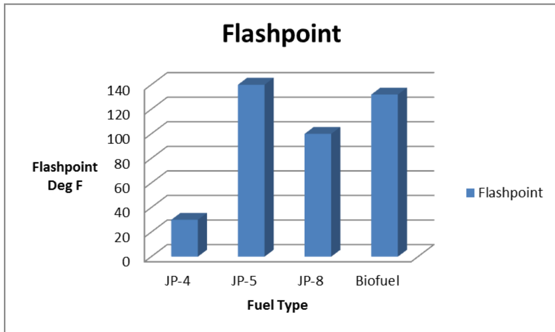
Figure 1. Jet Fuel Flashpoint Comparison (After Holmgren 2008 and Hovensha 2012)
