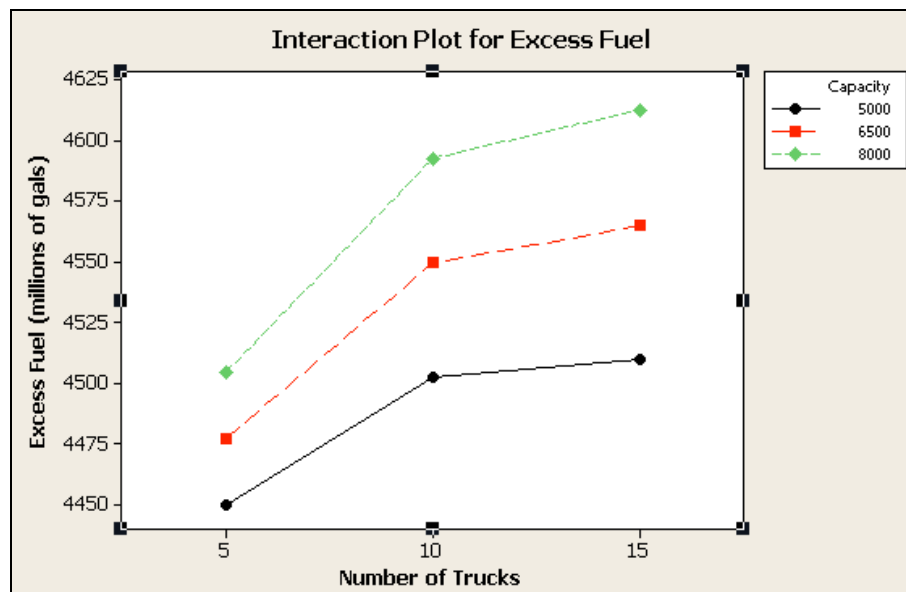
Figure 31. Interaction plot of Excess (millions of gallons) for the Combined Alternative
