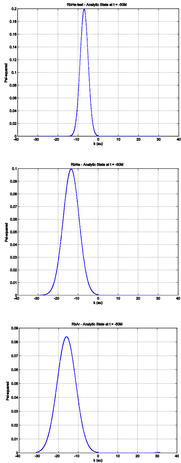
Fig. 3.10.2d: Intermediate Moller state in the momentum representation, for Rb + He (top), Rb + Ne (middle), and Rb + Ar (bottom). There is some leakage of the wavepacket into right-hand side of the grid for Rb + Ar that is a small source of error at high energy.
