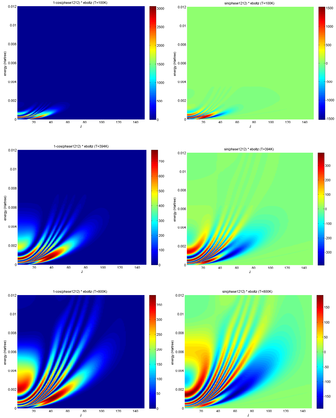
Fig. 2.5h: [1 - \cos \theta_J(E)] \times \text{Boltzmann distribution} (left) and \sin \theta_J(E) \times \text{Boltzmann distribution} (right) for the A^2\Pi_{1/2} state of the fully coupled case of Rb + He, at T = 100 K (top), T = 394 K (middle), and T = 800 K (bottom), top-down view. See (2.132b). These plots are shown primarily to compare with Fig. 2.5f. Their actual form is modified somewhat when used to calculate the shift coefficient, as discussed in section 2.6.
