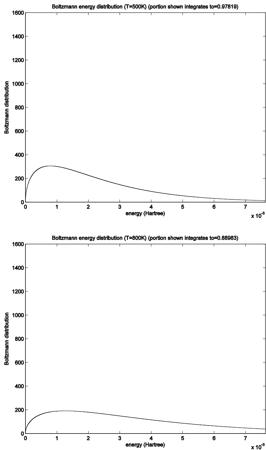
Fig. 3.10.3c: Boltzmann distribution at T = 500 K (top) and T = 800 K (bottom), for energies from E = 0 to E = 0.0075 Hartree. Note that at higher temperatures we truncate more of the total distribution if we stop integrating at E = 0.0075 Hartree.
