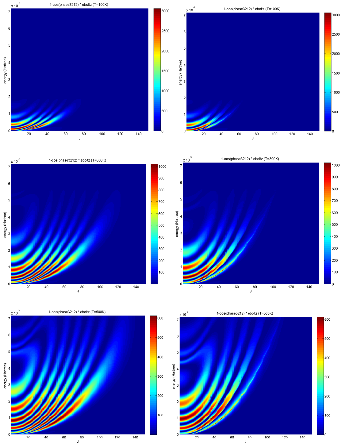
Fig. 3.10.3b: [1 - \cos \theta_j(E)] \times \text{Boltzmann distribution} for the \left| \frac{3}{2}, \frac{1}{2} \right\rangle state of the uncoupled case (left) and the fully-coupled 3x3 case (right) of Cs + He at T = 100 K (top), 300 K (middle), and 500 K (bottom), top-down view.
