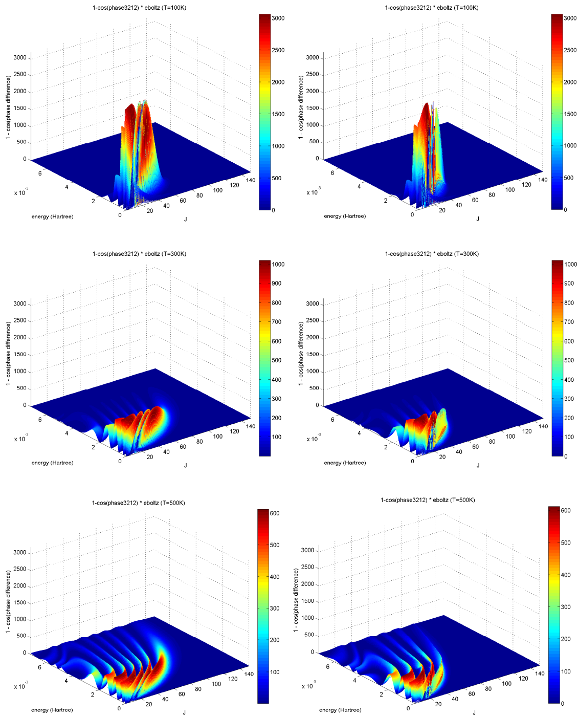
Fig. 3.10.3a: [1 - \cos \theta_j(E)] \times \text{Boltzmann distribution} for the \left| \frac{3}{2}, \frac{1}{2} \right\rangle state of the uncoupled case (left) and the fully-coupled 3x3 case (right) of Cs + He at T = 100 K (top), 300 K (middle), and 500 K (bottom).
