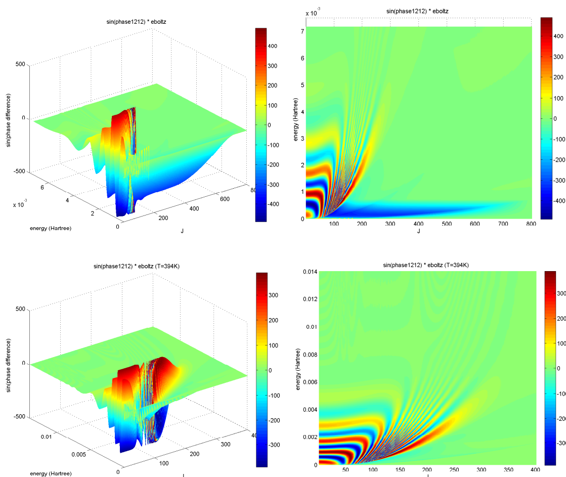
Fig. 3.10.2h: \sin \theta_j(E) \times \text{Boltzmann distribution} for the A^2\Pi_{1/2} state of the uncoupled case of Cs + Ar, at T = 394 K, side view (left) and top-down view (right). An early attempt (top) at generating the Moller states proved not to propagate far enough into the distant past. The latest run (bottom) propagates twice as far. Note that there are differences in scale between the runs. The feature appearing across the low-energy edge of the early run (top) is caused by the Moller state issue. Moller states in both data sets satisfied all the needs of the work of Lewis (Lewis, 2011), but give wholly inadequate scattering phase shift differences.
