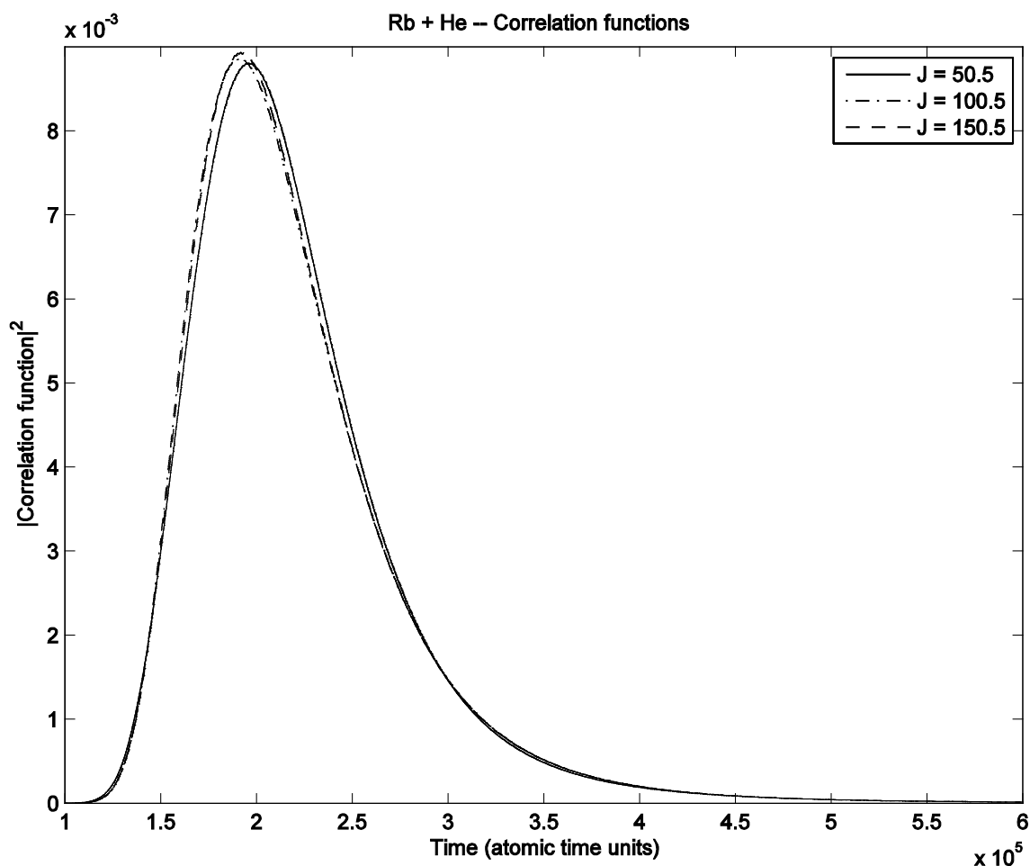
Fig. 2.4c: Squares of correlation functions for the A^2\Pi_{1/2} state of Rb + He.
