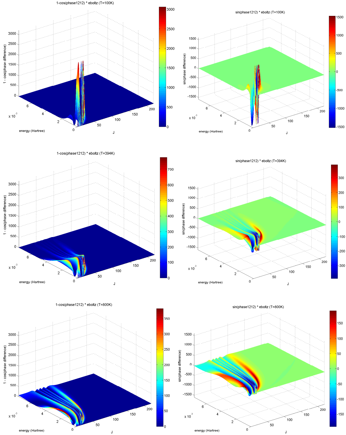
Fig. 2.5e: [1 - \cos \theta_J(E)] \times \text{Boltzmann distribution} (left) and \sin \theta_J(E) \times \text{Boltzmann distribution} (right) for the A^2\Pi_{1/2} state of the uncoupled case of Rb + He, at T = 100 K (top), T = 394 K (middle), and T = 800 K (bottom), side view. See (2.132c).
