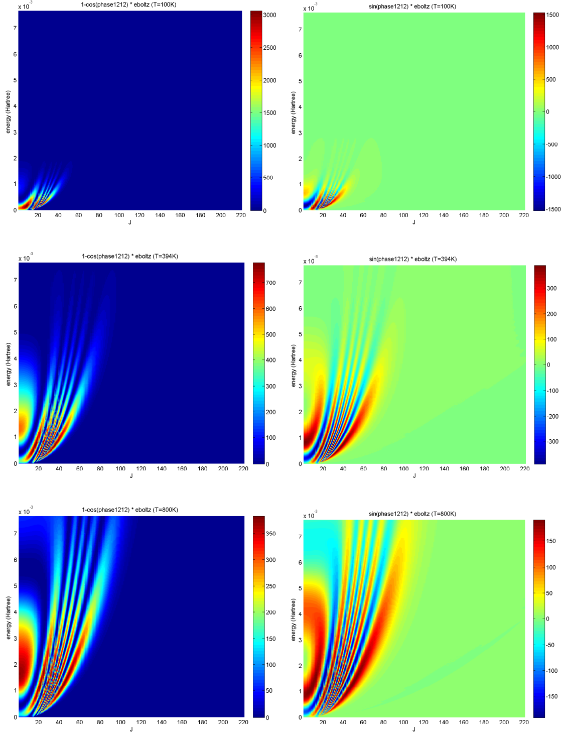
Fig. 2.5f: [1 - \cos \theta_J(E)] \times \text{Boltzmann distribution} (left) and \sin \theta_J(E) \times \text{Boltzmann distribution} (right) for the A^2\Pi_{1/2} state of the uncoupled case of Rb + He, at T = 100 K (top), T = 394 K (middle), and T = 800 K (bottom), top-down view. See (2.132c).
